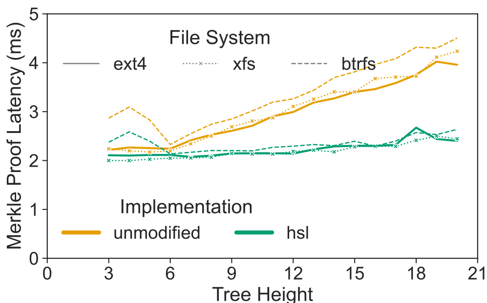
Figure 6.13: Evaluating merkle proofs: The figure shows the time taken in milliseconds (y-axis) to validate a merkle proof on merkle trees of different depths (x-axis). We compare two implementations, with and without HSL differentiated by color. We run the workload on ext4, XFS, and btrfs differentiated by line styles.
