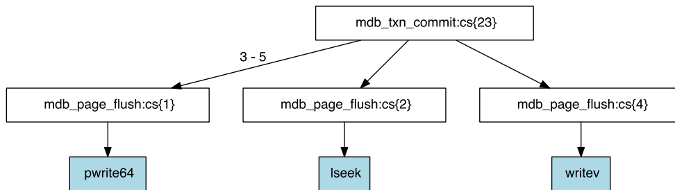
Figure 4.1: Visualizing portions of LMDB with Ikhnaie: We start with an observation of repeated pwrite64 syscalls and ask Ikhnaie to give us a visualization of that region. Ikhnaie first focuses on that region to identify the system calls and functions, and then scans the entire log to provide information on that region for the entire workload. In the above call-graph visualization, the leaves (colored) correspond to system calls. Every other node is a call site, i.e., a function name and a position within the function. In this figure, all three system calls are invoked by the same function ( mdb_page_flush ) at different call sites: cs{1} , {2} , and {4} . The figure also shows that cs{1} is invoked multiple times (3–5 times), followed by one lseek and one writev . All three call sites are invoked as part of a single execution of the mdb_txn_commit function. The image gives us context to decide whether we need to dig further. While not depicted, each of the nodes in the call graph are hyperlinked to the source location, allowing us to immediately take a look at the source code. In this specific case, LMDB maintains a list of dirty pages (pages that are modified during a transaction) that need to be flushed to disk. As LMDB keeps track of dirty pages in sorted order, sometimes the dirty pages are contiguous, leading to an lseek() and a single writev() . In other cases, each non-contiguous page can be written out with a pwrite() . Upon source-code inspection, we also notice pre-processor macros that depend on compile time flags. For example, building with MDB_USE_PWRITEV changes the pattern to always have one leaf pwritev() repeated multiple times.
