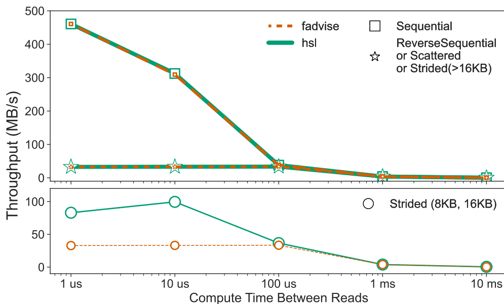
Figure 6.6: Comparing HSL .expect hint with always issuing fadvise(): The figure shows two graphs divided based on access pattern. In both graphs, the color identifies the application being used: always fadvise, or .expect with hsl. The markers represent access patterns. The top graph contains results for sequential, reverse sequential, scattered, and large strided (more than 16KB strides) access patterns. Sequential uses the square marker while the remaining three have the same results denoted by the star marker. The bottom graph contains results for small strided access patterns (8KB or 16KB) denoted by a circle marker. The y-axis (different for top and bottom) measures the throughput, and the x-axis (shared) varies the compute time between reads.
