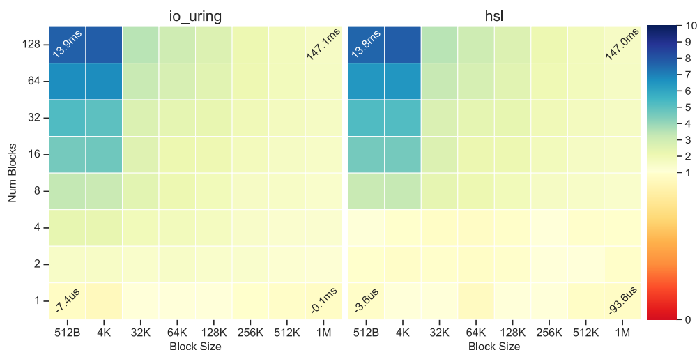
Figure 6.8: Evaluating scattered uncached reads on ext4: The figure shows the speedup obtained by two implementations over using traditional pread() system calls to perform scattered reads on a file that is not in the page cache. On the left is an implementation that always uses io_uring , while the right uses HSL which selectively uses io_uring . In each graph, the x-axis represents the size of every chunk (Block Size) in the scattered read while the y-axis represents the number of chunks (Num Blocks) in the scattered read. The color of each cell represents the speedup (greens and blues) or slowdown (oranges and reds) over the system call implementation. We annotate the boundaries with the difference to the system call implementation: the speedups (positive) or slowdowns (negative) are in microseconds for fewer chunks while in milliseconds for larger number of chunks.
