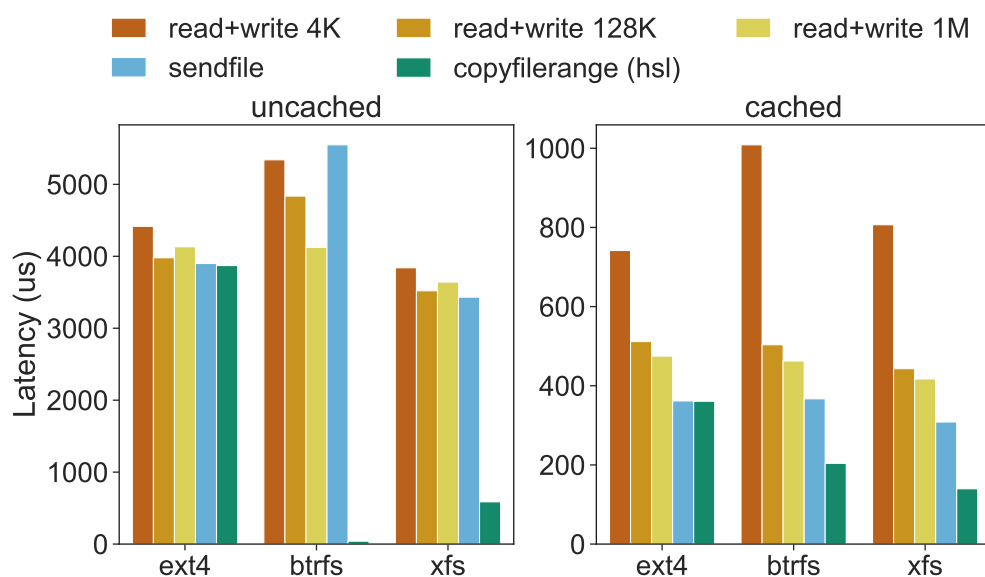
Figure 6.1: Evaluating implementations to copy 1MB to an existing file on different file systems: The figure shows the per page latency in microseconds (y-axis) for different local file systems (x-axis) performing a copy with different implementations. The two graphs correspond to whether the files were in the page cache (right: cached) or not (left: uncached).
