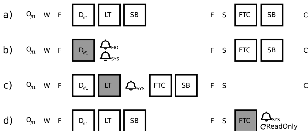
Figure 3.8: Blockviz traces for w_{su} on btrfs:
