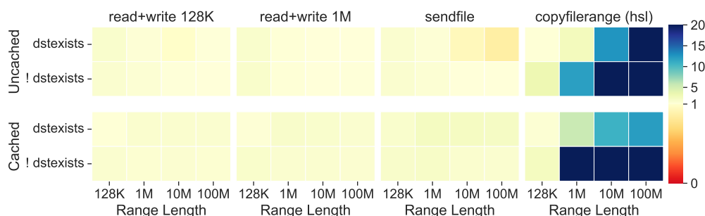
Figure 6.2: Evaluating implementations of large single-range copies on XFS: The figure shows the speedups of each copy implementation (four columns) relative to the read+write implementation using a 4KB buffer. The fourth column represents both copy_file_range and HSL. The two rows correspond to whether the files are uncached (top) or cached (bottom). Inside each heatmap, the y-axis represents whether the destination file exists or not ( dstexists and !dstexists ). The x-axis varies the length of the range being copied.
