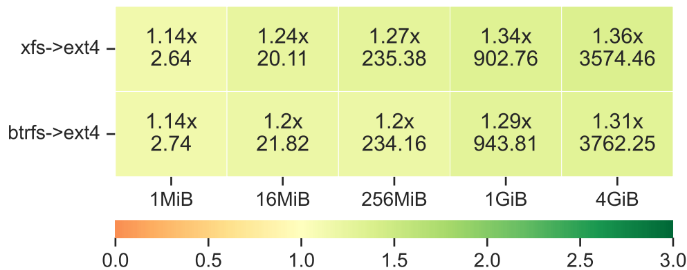
Figure 6.11: Evaluating coreutils cp on different file systems: The figure shows the speedup obtained by using a modified version of coreutils cp that uses HSL over the unmodified version, when the source file is cached. On the x-axis, we vary the size of the file. On the y-axis, we vary source and destination file systems. Each cell is colored according to the speedup and is also annotated accordingly on the first line. The second line in each cell is the time taken by the unmodified version (in microseconds) to perform the copy.
