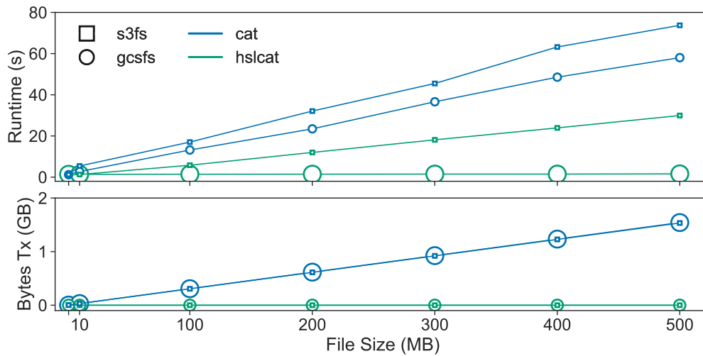
Figure 6.5: Evaluating file concatenation on remote object storage: The figure shows the time taken to concatenate three equal sized files into one on S3 and GCS, using cat and HSL. We vary file size on the x-axis, measure runtime in seconds (top y-axis), and measure bytes transferred (bottom y-axis).
