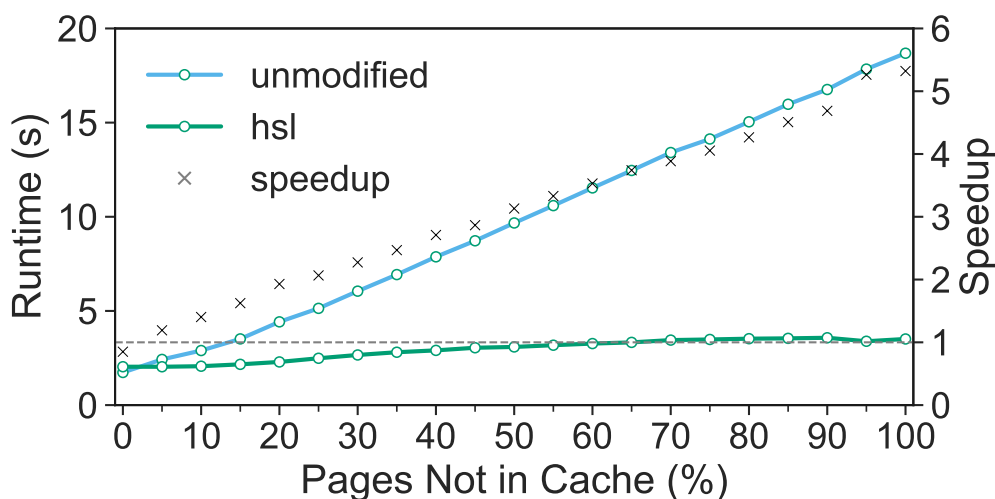
Figure 6.15: Evaluating TPC-H query 6 with SQLite on ext4: The figure shows the time taken in seconds (left y-axis) to execute the query on a database that has some pages in the cache (x-axis). We compare two implementations: unmodified SQLite and SQLite with HSL, differentiated by color. The right y-axis shows the speedup obtained when using SQLite with HSL. At x=0 , all pages are in the cache, and the two implementations are nearly identical; the unmodified version is slightly faster. However, with even 5% uncached pages, HSL outperforms the unmodified version.
