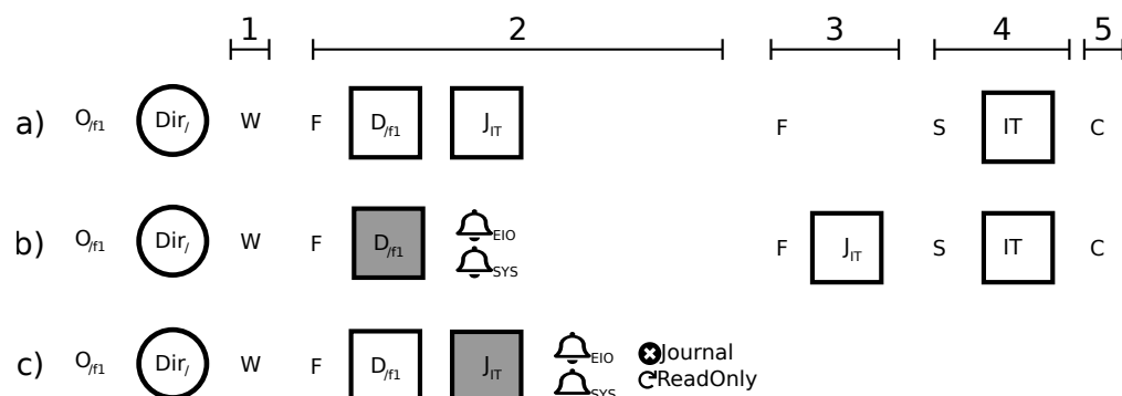
Figure 3.2: Blockviz traces for w su on ext4 ordered mode:
