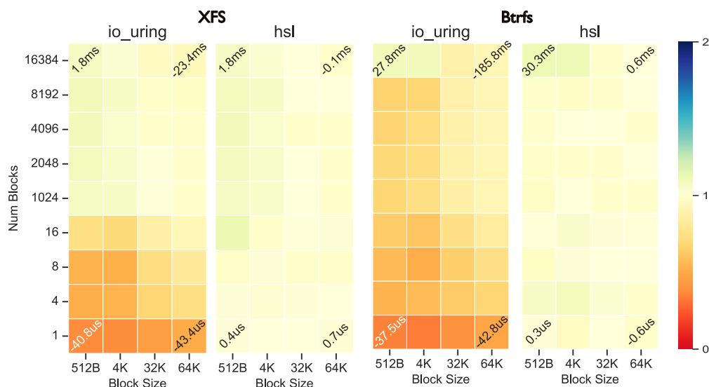
Figure 6.10: Evaluating scattered writes on XFS and btrfs: The figure shows four heatmaps similar to figure 6.9, but for scattered writes on XFS and btrfs. As HSL is aware of the performance equilibrium between io_uring and system call implementations for writes on XFS and btrfs, it sets different thresholds accordingly. HSL uses system calls for fewer than 1024 scattered reads in XFS but 16384 scattered reads in Btrfs. For larger chunk sizes (32K or more), HSL always uses system calls as the cost of copying data becomes the bottleneck.
