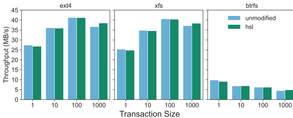
Figure 6.14: Evaluating update operations to LMDB: The figure shows the throughput measured in MB/s (y-axis) for a 100% update workload. We vary the number of update operations within a transaction (x-axis). We compare two implementations: LMDB with HSL, and an unmodified LMDB differentiated by color. We run LMDB on three file systems: ext4, xfs, and btrfs as indicated above each graph.
