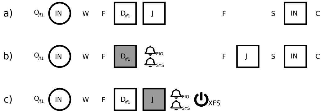
Figure 3.6: Blockviz traces for w_{sll} on XFS:
