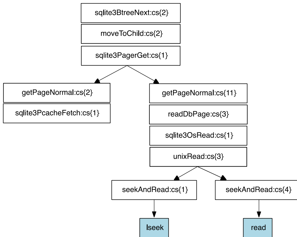
Figure 4.2: Visualizing portions of SQLite with Ikhnaie: We observed repeated patterns of lseek() followed by read() when running SQLite. At first, we were unsure whether multiple lseek-read pairs appear together or one at a time. With Ikhnaie, the visualization tells us that every pair appears one at a time and is the result of a sqlite3BtreeNext function call. As observed in the figure, the system calls are hidden under a layer of one-to-one portability abstractions: sqlite3OsRead , unixRead , followed by seekAndRead . With the help of Ikhnaie, SQLite design documents, and source code, we learn the following: SQLite uses B-Tree data structures whose nodes are called “pages”, and rows in a database table reside in B-Tree leaf pages. SQLite uses sqlite3BtreeNext to move to the next row, which may be on the same page or on a different page. If the new page is in the page cache (left subtree in the figure), no file-system interaction is necessary. If the page has to be read from disk, the code takes the right subtree path resulting in a single lseek() and read() to the target page. As with LMDB in Figure 4.1, a compile-time flag ( USE_PREAD ) changes this behavior to use a single pread() instead.
