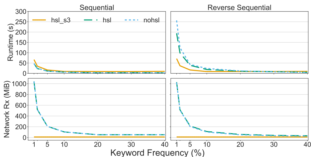
Figure 6.7: Comparing .filter and .filter_endpoint against a traditional filter workload: The figure shows four graphs divided into two columns based on access pattern (left:sequential and right:reverse sequential), and into two rows based on metric captured (top: runtime in seconds, bottom: bytes received over the network in MB). The colors of each line represent different applications: filtering without hsl (nohsl), filtering with hsl locally (hsl), filtering with remote compute through aws lambda (hsl_s3). All graphs use the same x-axis which denotes the frequency of the keyword used for the filter workload. The y-axis denotes the metric captured (top:runtime, and bottom: bytes received).
