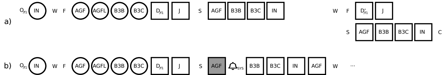
Figure 3.7: Blockviz traces for w_{m.a} on XFS:
