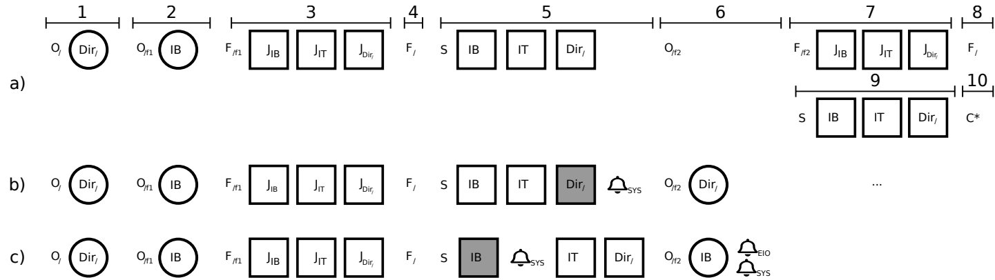
Figure 3.4: Blockviz traces for w_{dir} on ext4 ordered mode:
