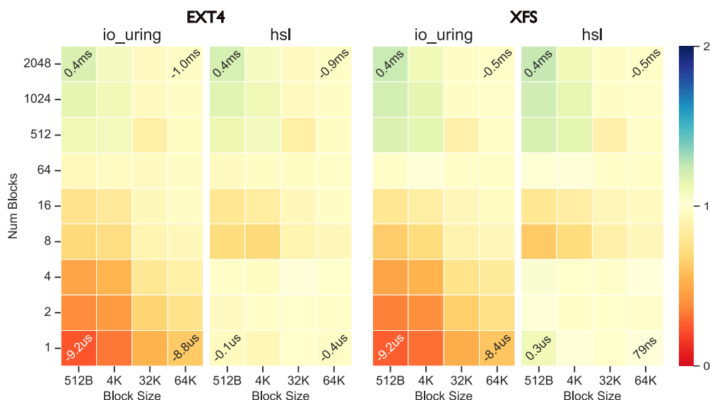
Figure 6.9: Evaluating scattered cached reads on ext4 and XFS: The figure shows four heatmaps that identify speedups and slowdowns of two scattered read implementations over traditional pread() system calls over a file that is fully in the page cache. Each half represents a different file system: ext4 and XFS respectively, and can be interpreted similar to Figure 6.8. As HSL is aware of poor cached read performance through io_uring , it uses the system call implementation for the smaller number of chunks.
