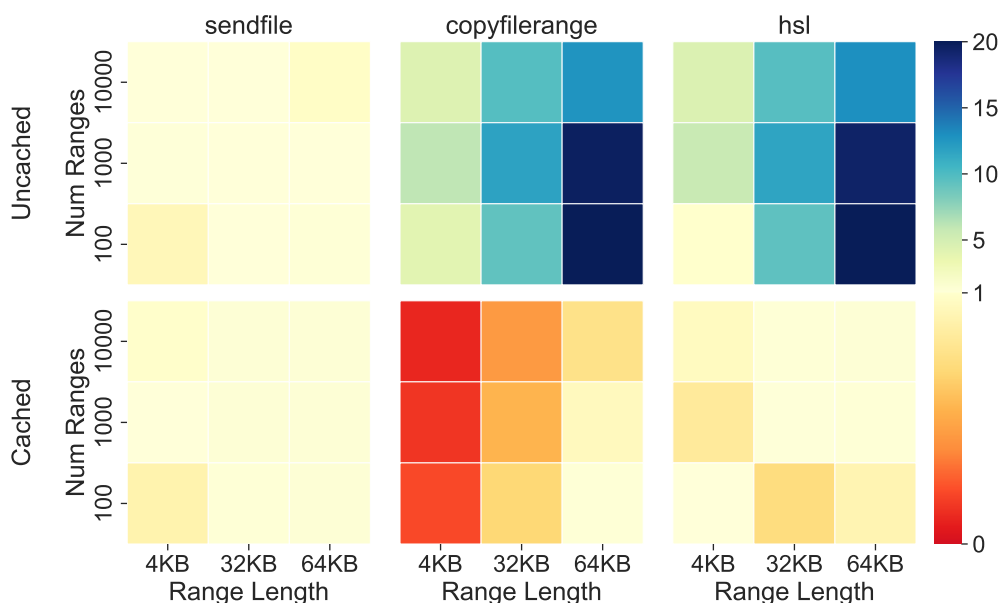
Figure 6.4: Evaluating implementations of small multi-range copies on XFS: The figure shows the speedups of each copy implementation (three columns) relative to the read+write implementation. The two rows correspond to whether the files are uncached (top) or cached (bottom). Inside each heatmap, the y-axis represents the number of ranges in the copy and the x-axis the length of each range being copied.
