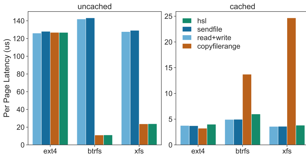
Figure 6.3: Evaluating implementations to copy 1000 4KB pages on different file systems: The figure shows the per page latency in microseconds (y-axis) for different local file systems (x-axis) performing a copy with different implementations. The two graphs correspond to whether the files were in the page cache (right: cached) or not (left: uncached).
