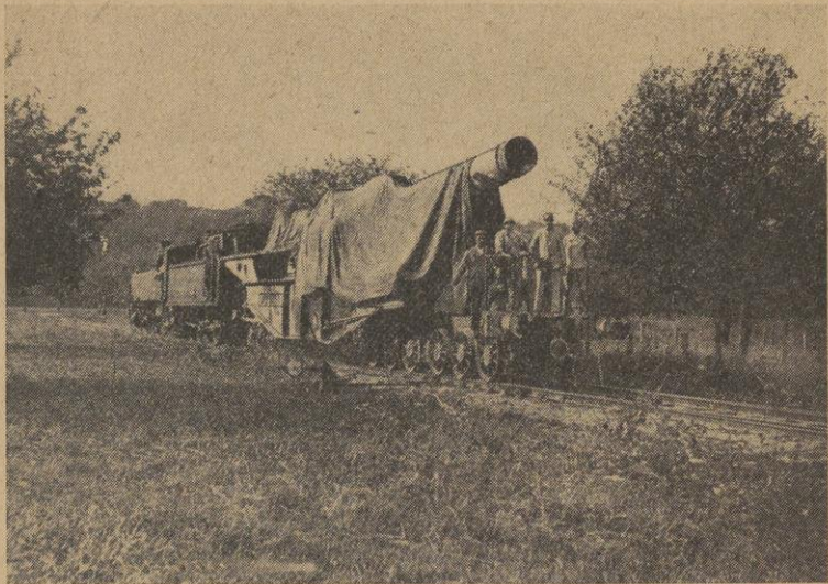
The 400 \frac{m}{m} (15.8 inch) howitzer.
