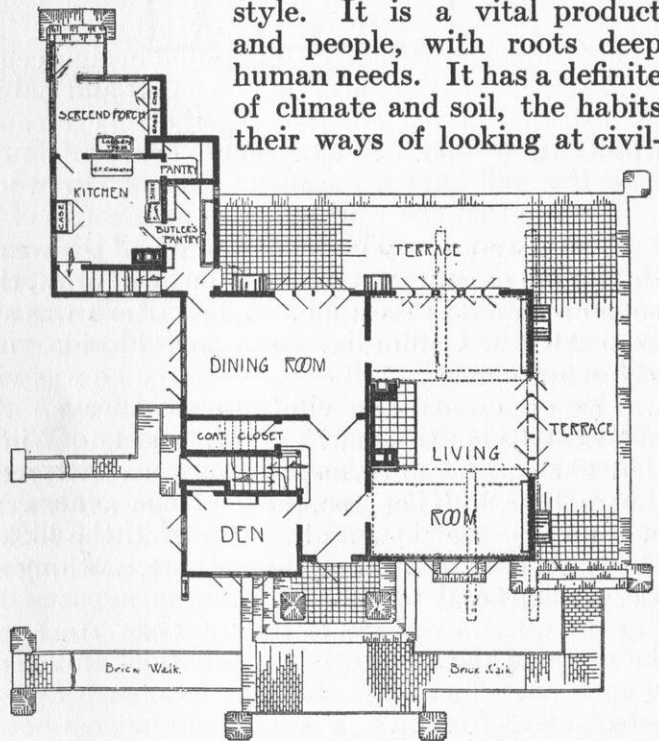
FIRST FLOOR PLAN FOR MR. PITCAIRN'S HOUSE: SEE PAGES 538 AND 539.
