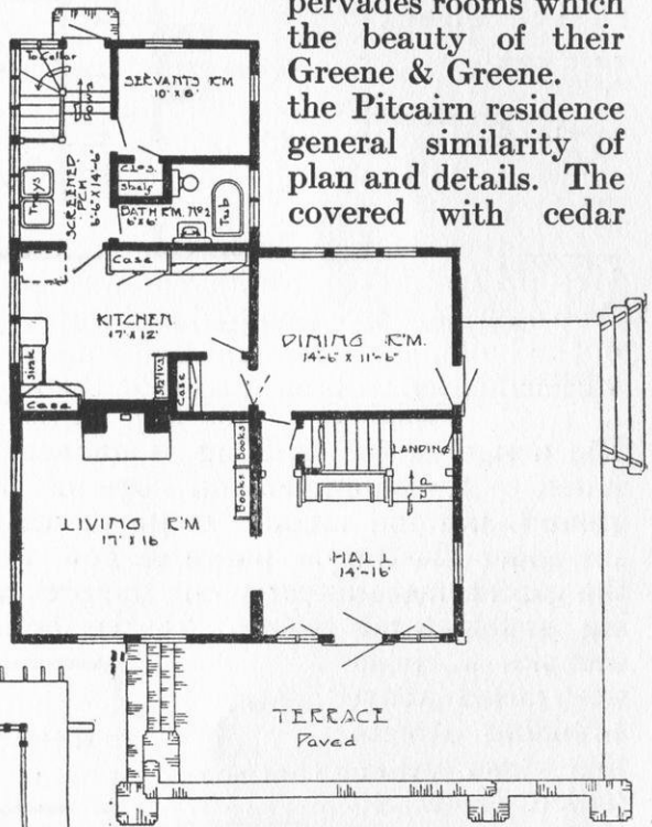
FIRST FLOOR PLAN OF MISS RANNEY'S HOUSE: SEE PAGE 541.
