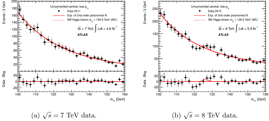
Figure 9.1: The diphoton invariant mass spectrum for selected events in the unconverted, central, low- p_{Tt} category for 2011 and 2012 data.
