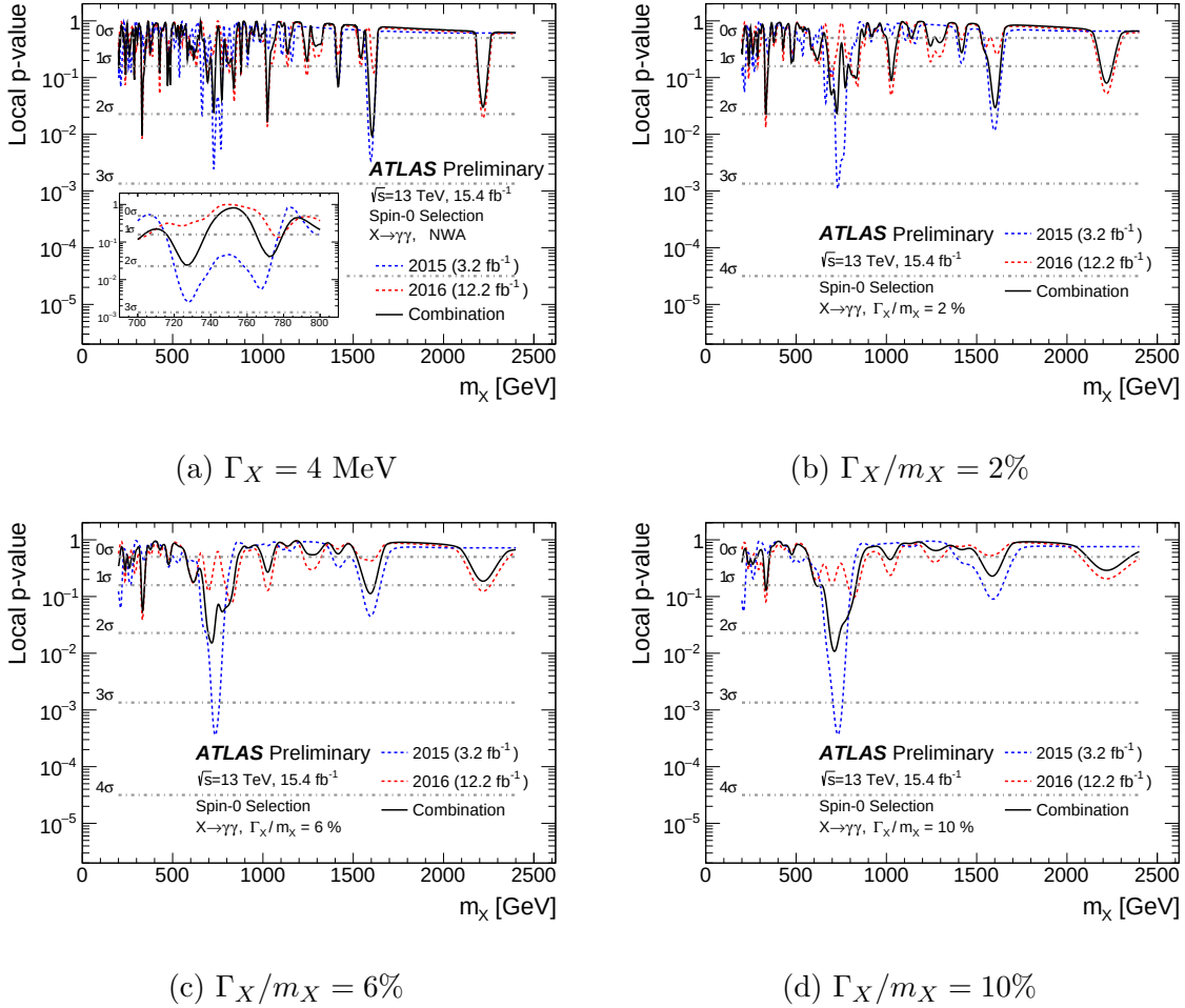
Figure 9.23: p_0 scans showing the compatibility of the observed data with the background-only hypothesis as a function of the mass of hypothetical scalar signals. Results are shown for four signal width hypotheses, including the narrow-width approximation, where \Gamma_X = 4 \text{ MeV} (Figure 9.23a), \Gamma_X/m_X = 2\% (Figure 9.23b), \Gamma_X/m_X = 6\% (Figure 9.23c), and \Gamma_X/m_X = 10\% (Figure 9.23d).
