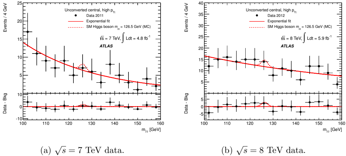
Figure 9.2: The diphoton invariant mass spectrum for selected events in the unconverted, central, high- p_{Tt} category for 2011 and 2012 data.
