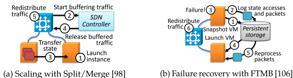
Figure 4.1: Scaling and failure recovery process with recently state management frameworks
