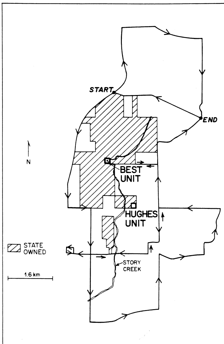
FIGURE 4. The 46-km cottontail roadside transect surrounding the Brooklyn Wildlife Area.
