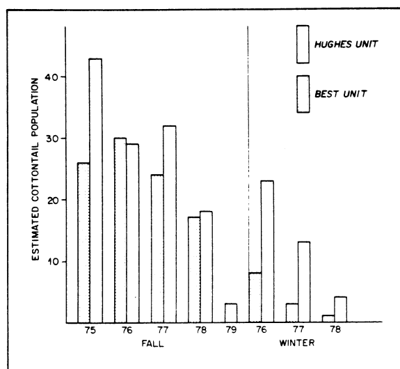
FIGURE 7. Cottontail population estimates derived from trapping results obtained at the Best and Hughes Units, 1975-79.
