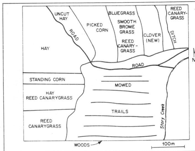
FIGURE 2. Best Experimental Unit (20 ha) (left) and Hughes Control Unit (20 ha) (right) in spring 1976 before treatment.
