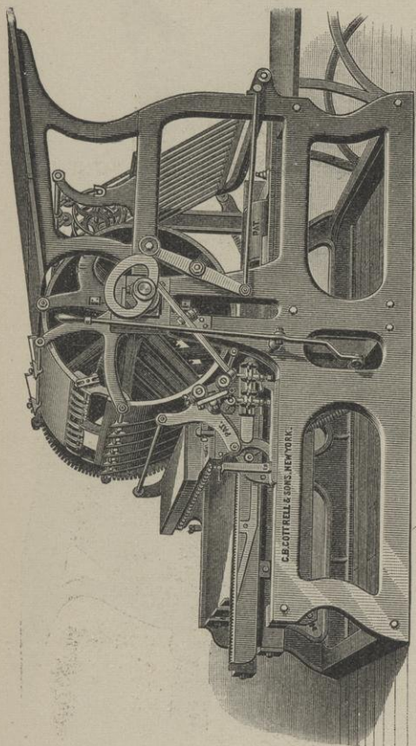
COTTRELL AIR-SPRING COUNTRY PRESS.
