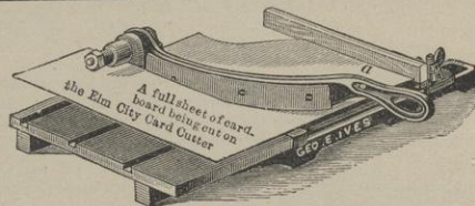
ELM CITY CARD CUTTER.
