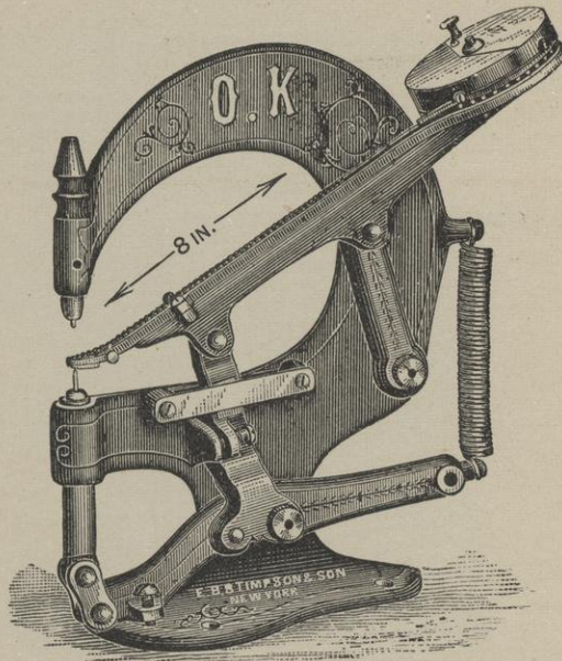
"O. K." SELF-FEEDING FOOT-POWER EYELETING MACHINE.
