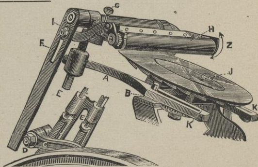
FRANKLIN INK FOUNTAIN.
