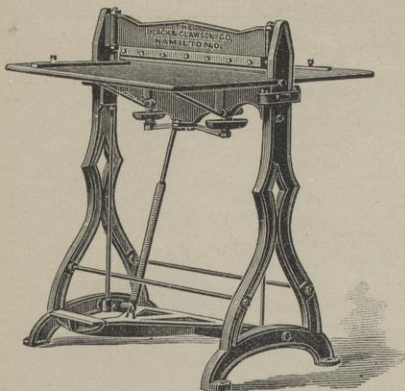
BLACK & CLAWSON PERFORATING MACHINE.
