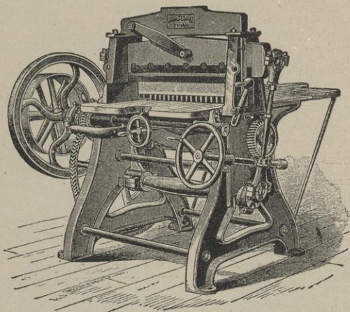
BROWN & CARVER IMPROVED PAPER CUTTER.
