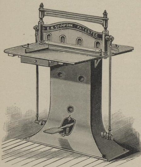
STIMPSON PERFORATING MACHINE.
