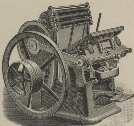
THE UNIVERSAL PRESS.
