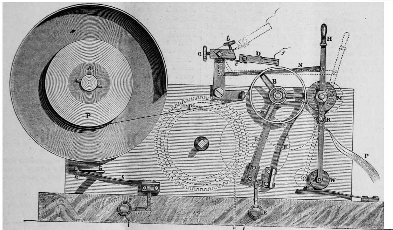
FIG. 25.—Alexander Bain's Automatic Chemical Printing Telegraph, 1846.
