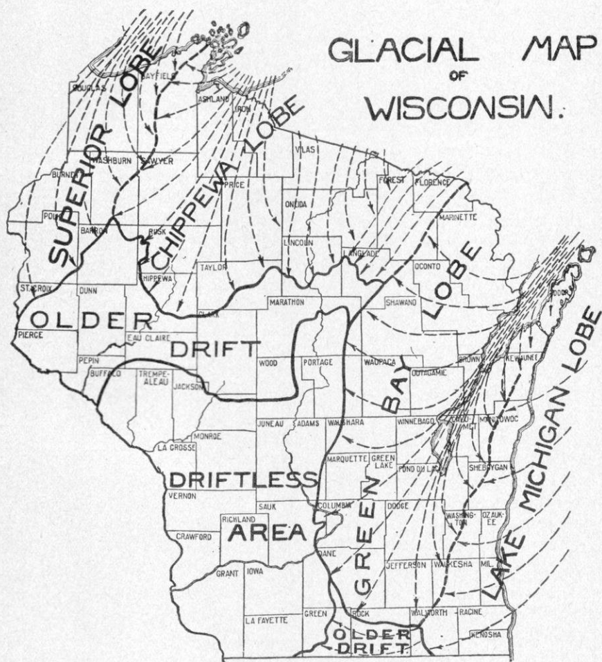
Fig. 7.—Map showing portions of Wisconsin covered by glacial soil or drift, and lines showing direction of movement of the ice in the different lobes or tongues.
