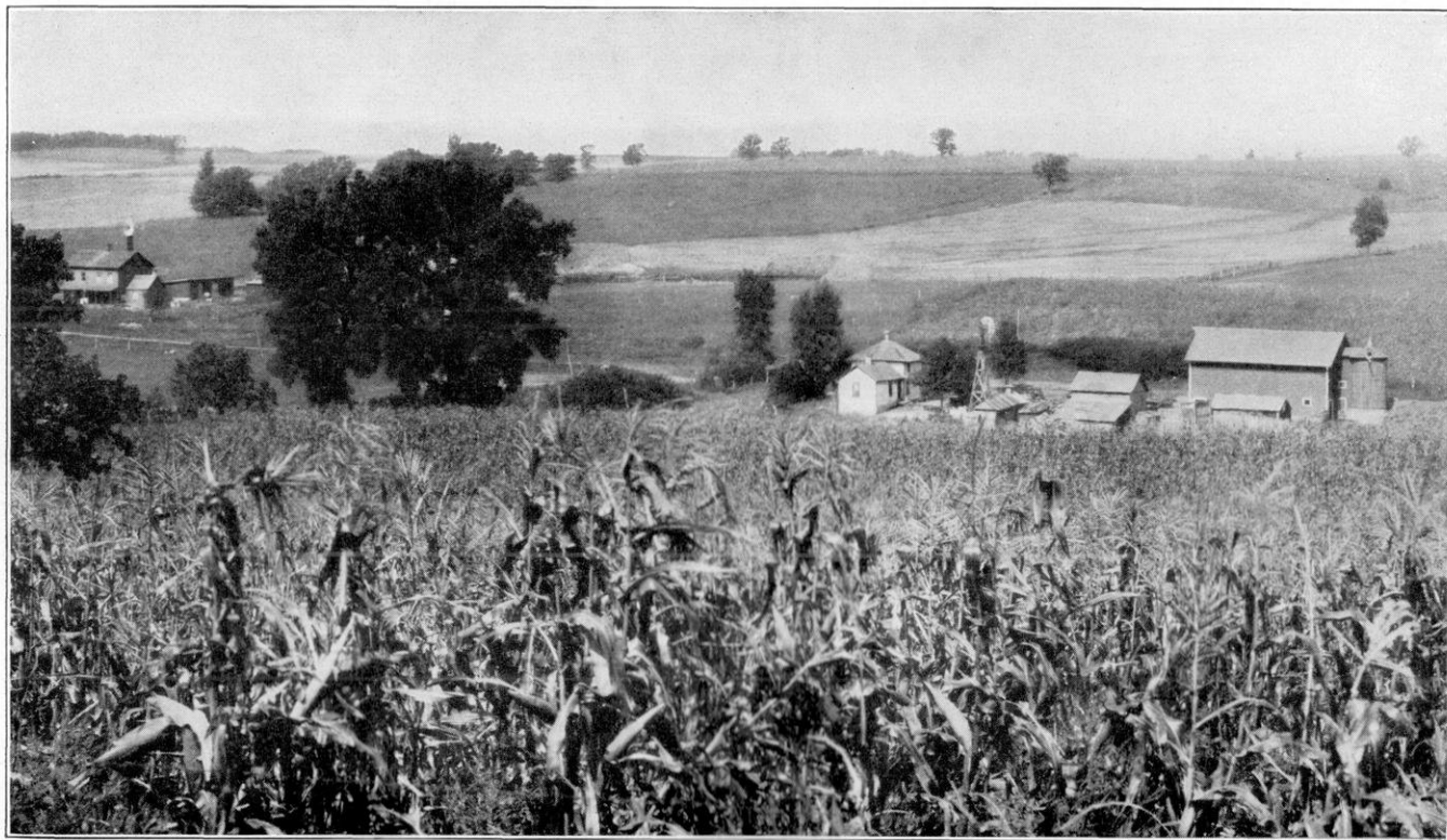
Plate XIV. View on Miami fine sandy loam in Columbia County.
