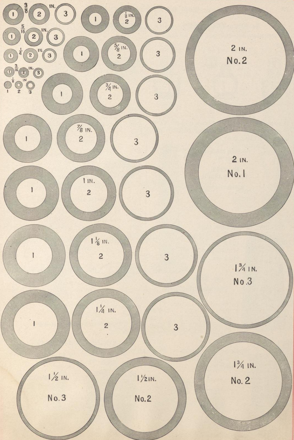
Diagram showing approximate thickness of walls and diameters of Glass Tubing. See No. 2285, page 70.
