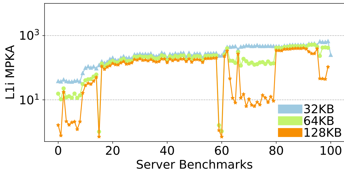
Figure 3.3: Varying L1i Size
