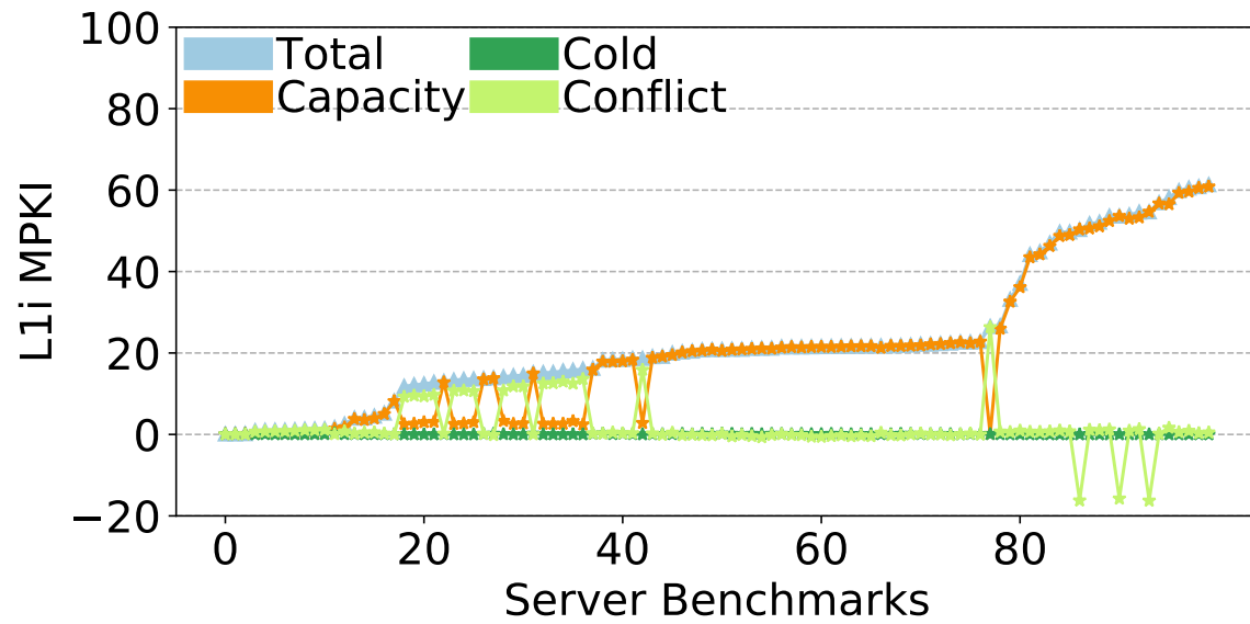
Figure 2.5: L1i (64KB) MPKI Breakdown
