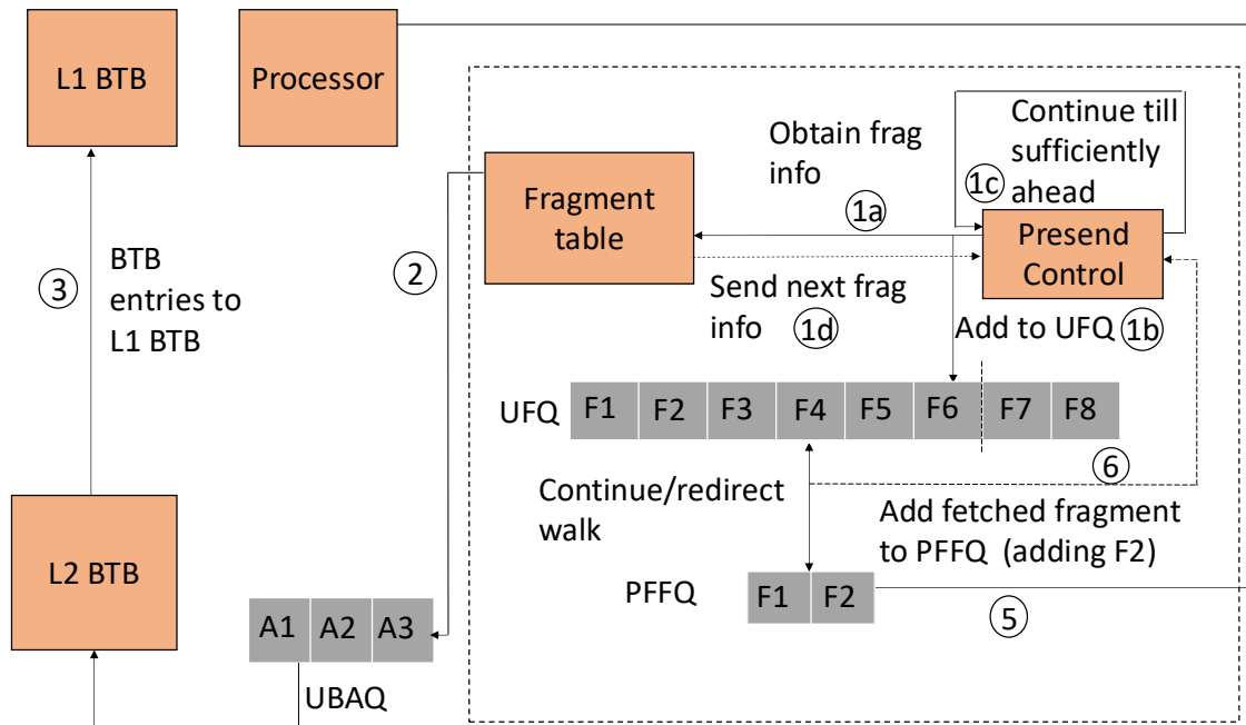
Figure 7.2: Instruction Presenting Unit (IPU) operation for BTB
