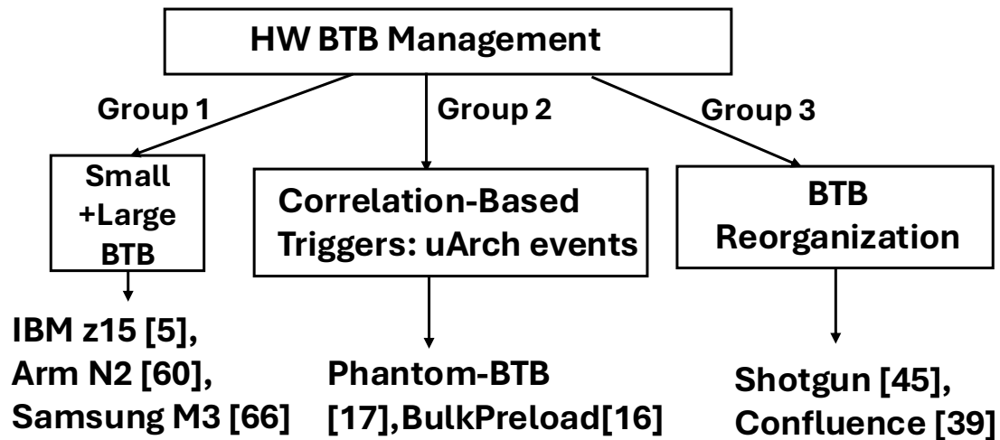
Figure 3.17: HW BTB Management Schemes
