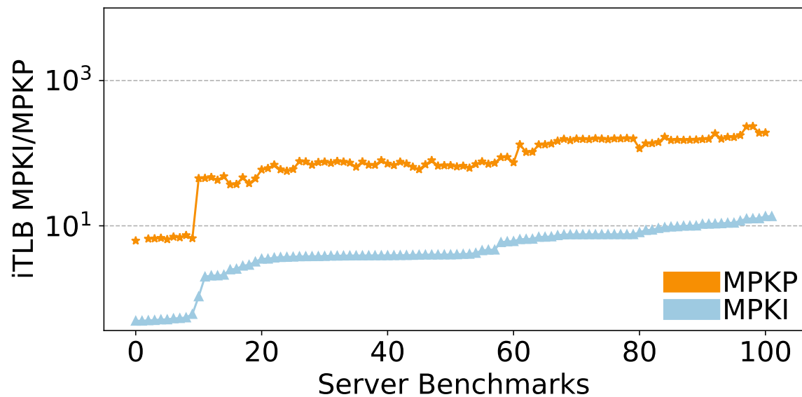
Figure 3.6: iTLB MPKI/MPKP
