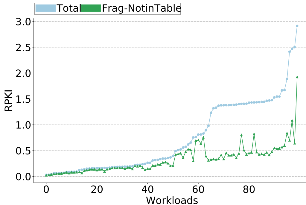
Figure 5.3: RPKI Components
