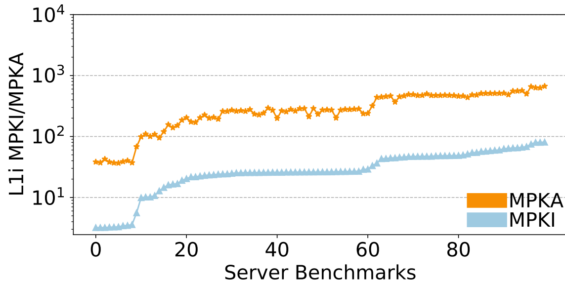
Figure 3.2: L1i MPKI/MPKA
