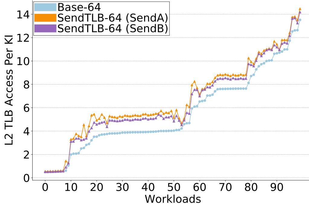
Figure 6.7: iTLB Traffic
