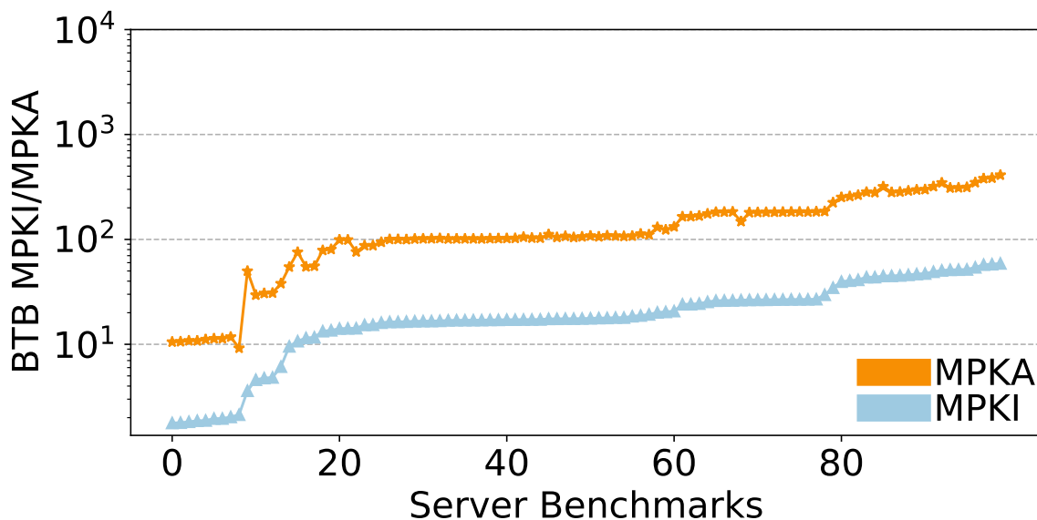
Figure 3.4: BTB MPKI/MPKA
