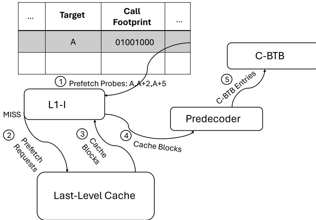
Figure 3.19: Shotgun Prefetching
