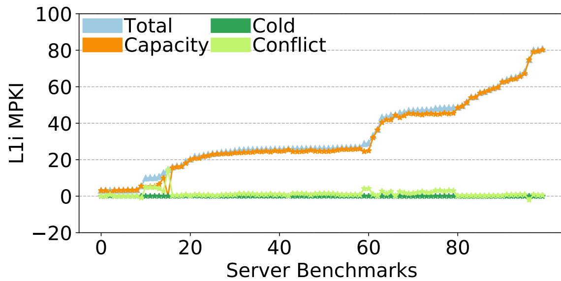
Figure 2.2: L1i (32KB) MPKI Breakdown
