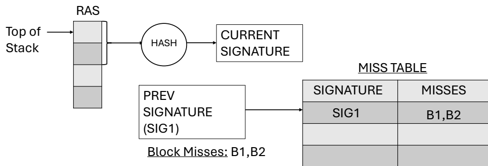
Figure 3.13: RDIP Datastructures
