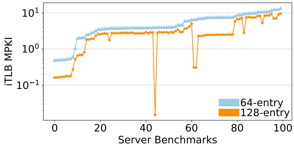
Figure 2.8: iTLB MPKI
