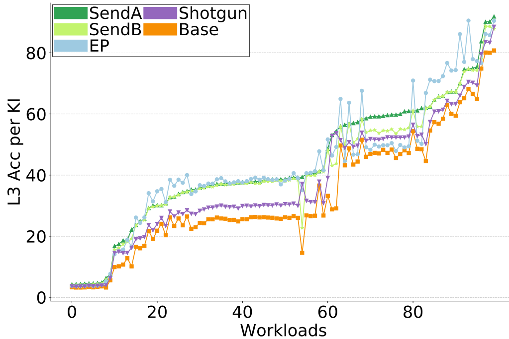
Figure 5.14: L1i Traffic
