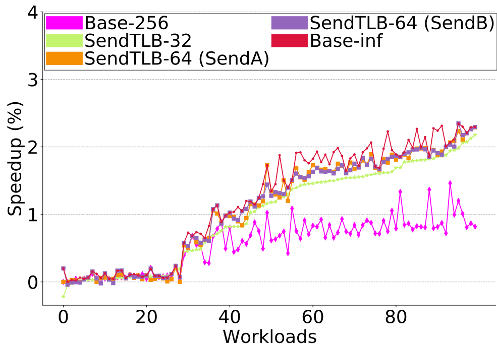
Figure 6.8: iTLB Speedup
