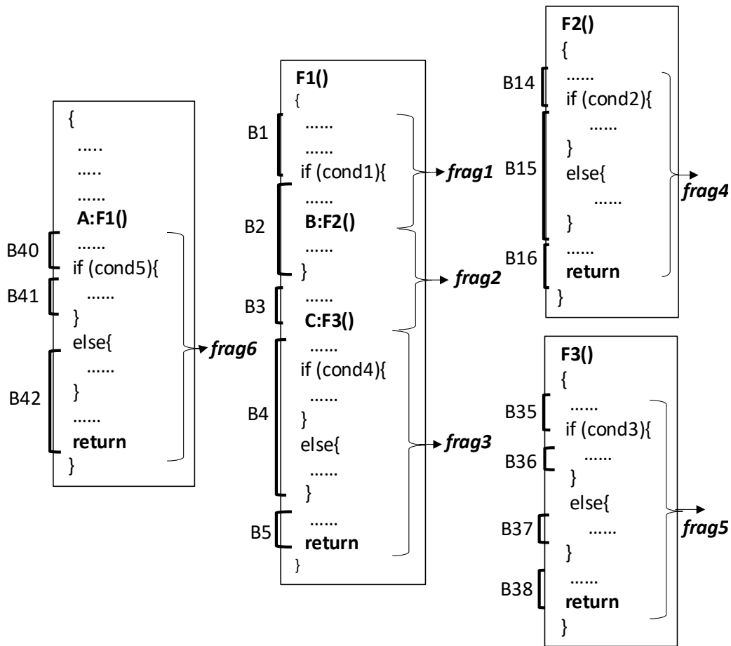
Figure 4.1: Fragments Example
