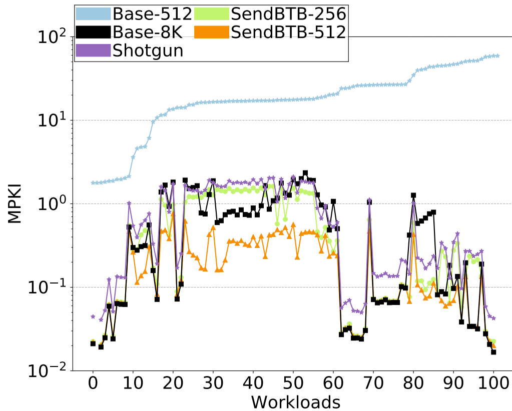
Figure 7.3: BTB MPKI
