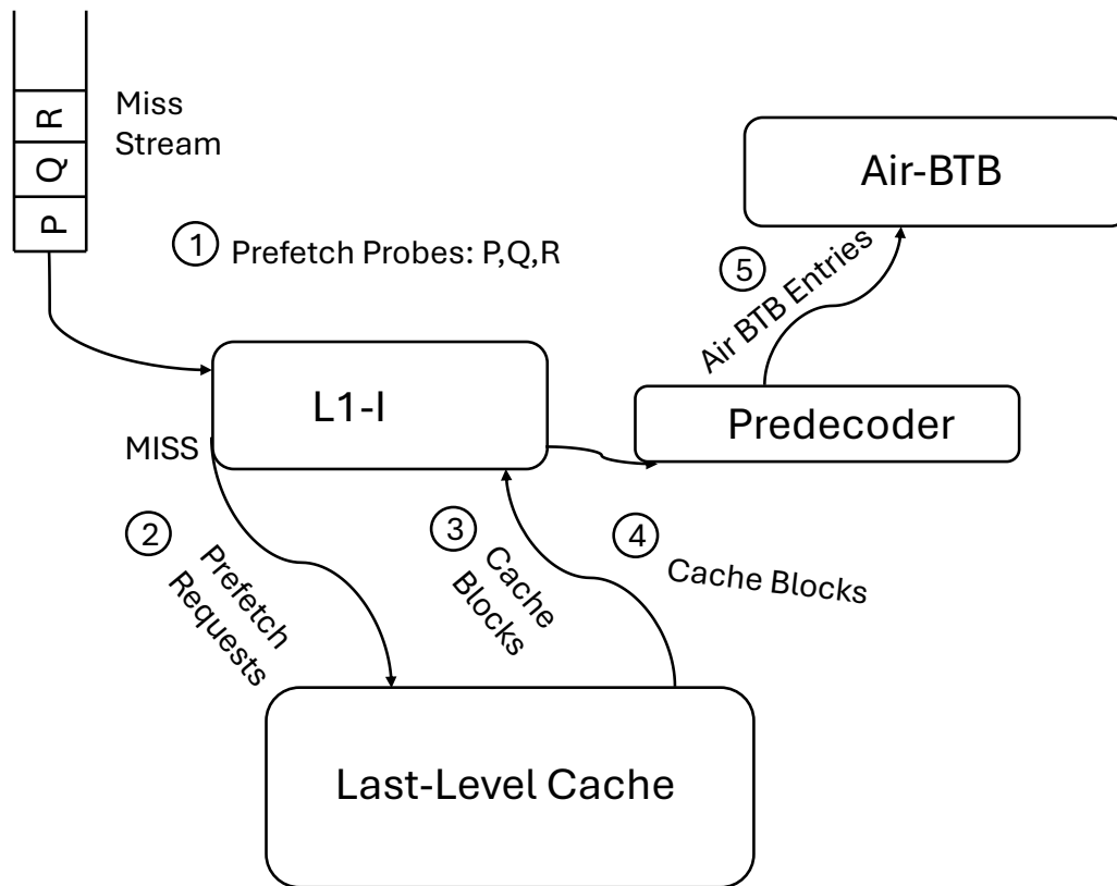
Figure 3.20: Confluence Operation
