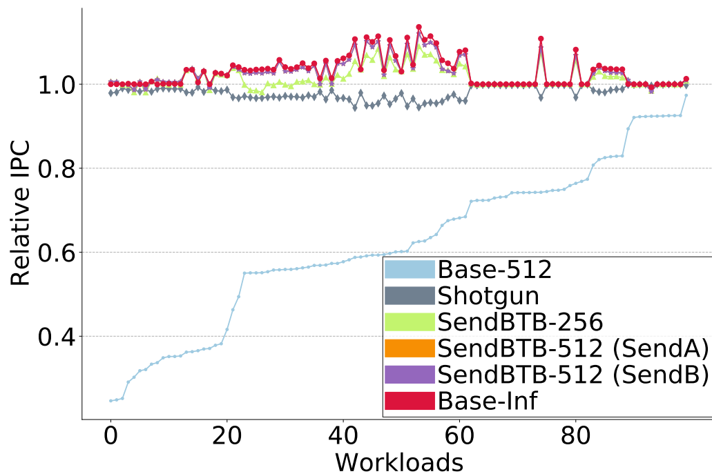
Figure 7.6: BTB IPC
