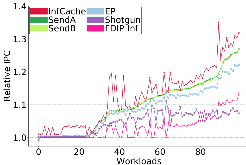
Figure 5.22: L1i IPC
