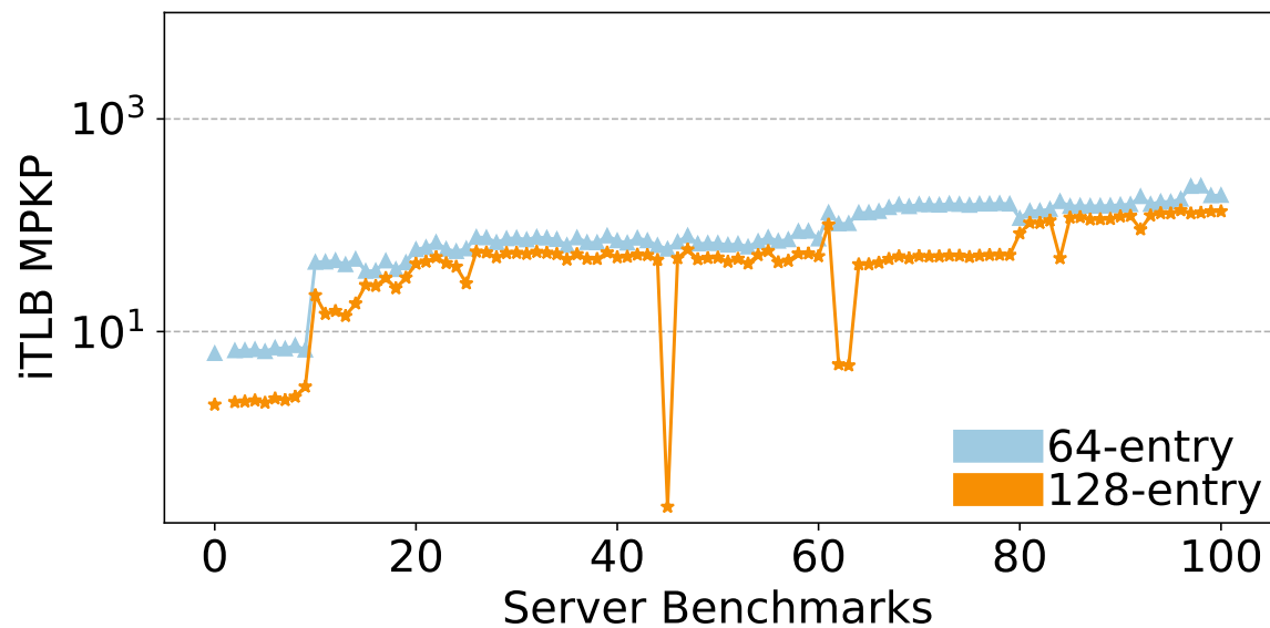
Figure 3.7: Varying iTLB Size
