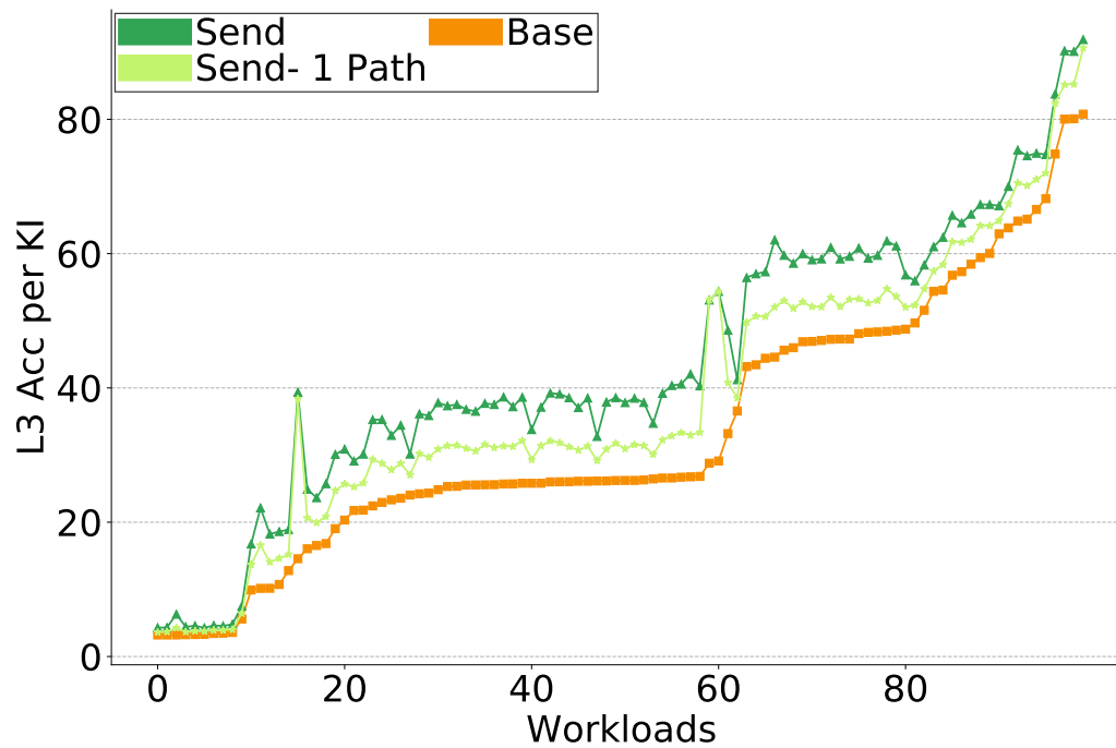
Figure 5.15: Traffic Breakdown
