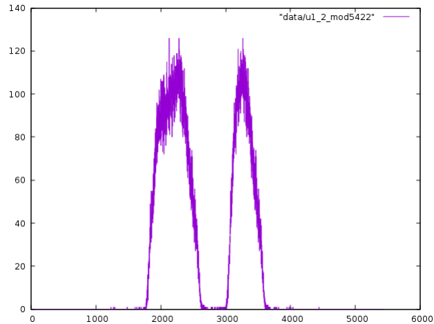
Figure 7: Distribution of U(1, 2) modulo \lambda
