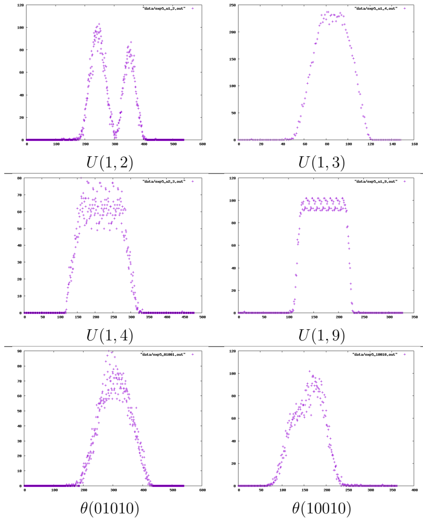
Figure 5: Distributions of various A modulo \lambda_A
