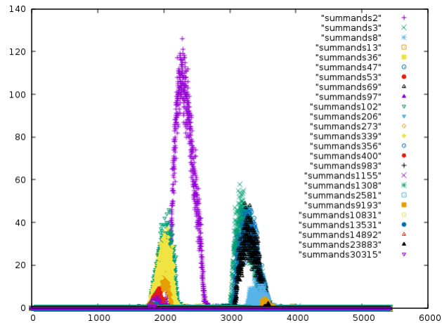
Figure 10: Distribution of all S_a for small summands a
