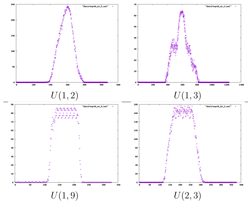
Figure 6: Numbers not in A nor in A + A plotted modulo \lambda_A
