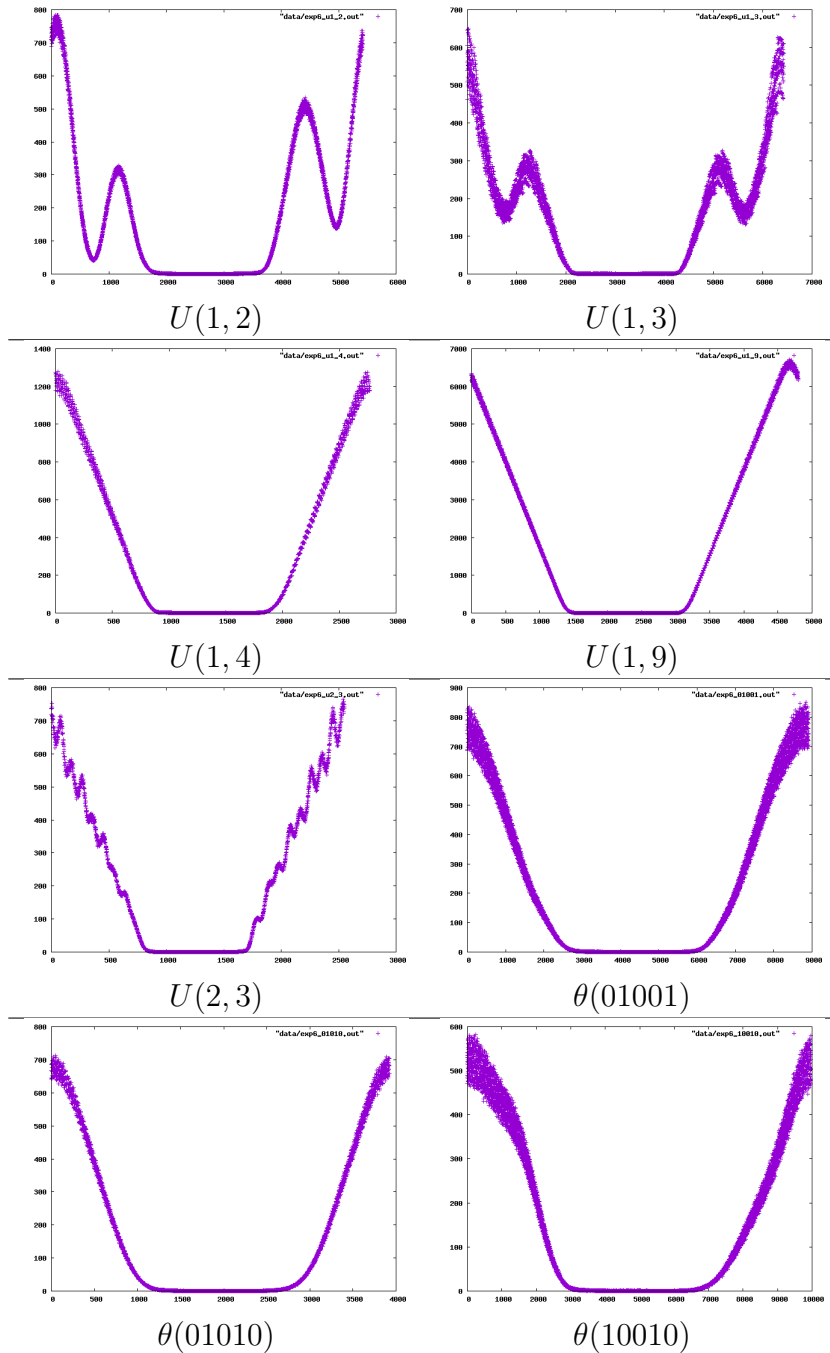
Figure 4: Plots of r_{A+A} modulo \lambda_A for various A
