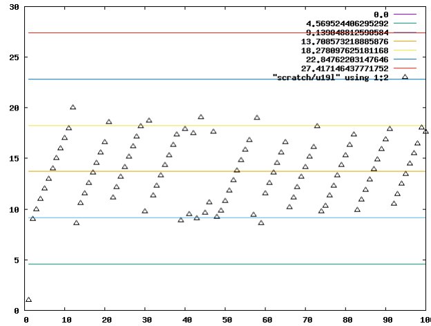
Figure 12: (n, a_n \bmod \lambda) for U(1, 9) and n \leq 100
