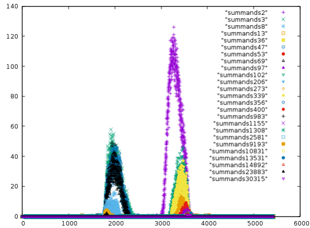
Figure 11: Distribution of S_a - a
