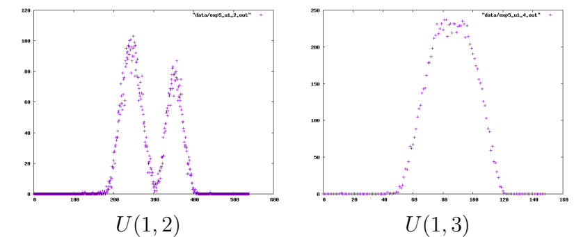
Figure 3: Some distributions of A \bmod \lambda_A
