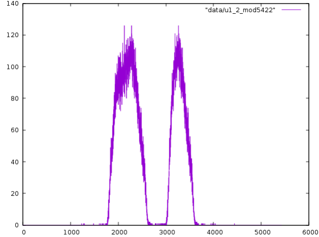
Figure 1: Distribution of A modulo \frac{2\pi}{\alpha}
