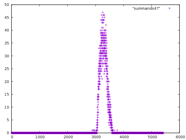
Figure 9: Distribution of S_{47}
