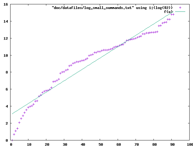
Figure 13: \log(s_i) for small summands s_i plotted against i
