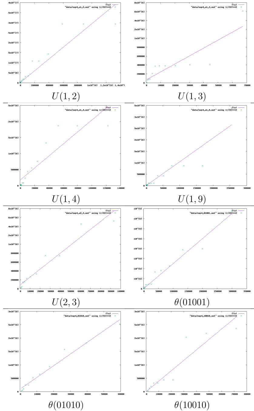
Figure 2: Plots of first d_N\alpha_A to violate conjectured decay rate.
