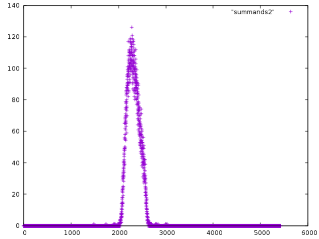
Figure 8: Distribution of S_2
