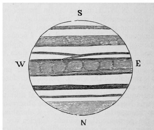
This sketch is copied from a drawing bearing the date of 1870, December 14 d 11 h 10 m . It may serve as an illustration of some of these remarks, though it makes but little pretension to accuracy.
