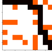
Figure 2.1: Optimal Policy Path.
