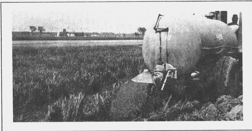
FIGURE 6. Discharging slurried waste in narrow swath from a tank wagon.
