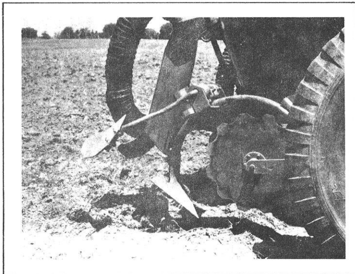
FIGURE 13. Sweep-shovel injectors with covering spoons.
