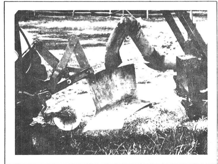
FIGURE 14. Sub-sod injection plow made from mold boards.
