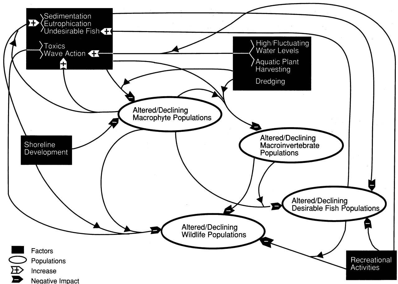
Figure A.1. The dynamics of ecosystem response: factors described in Appendix A that affect populations of aquatic macrophytes, macroinvertebrates, wildlife, and desirable fish in large, shallow lakes.
