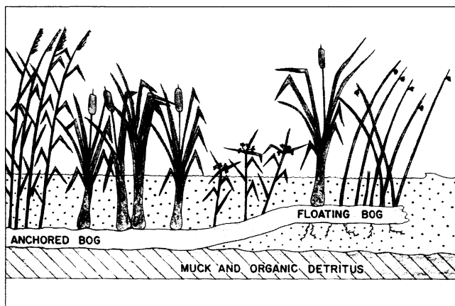
Figure 4. Floating bogs are created when (a) high and fluctuating water levels lift dense rhizomatous mats away from underlying substrates;
