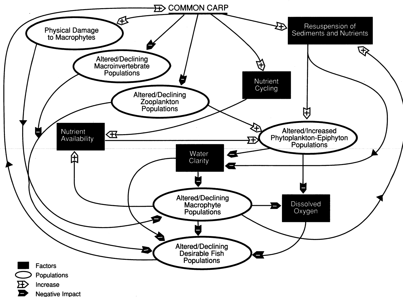
Figure A.2. Potential ecological impacts of carp on wetland ecosystems.
