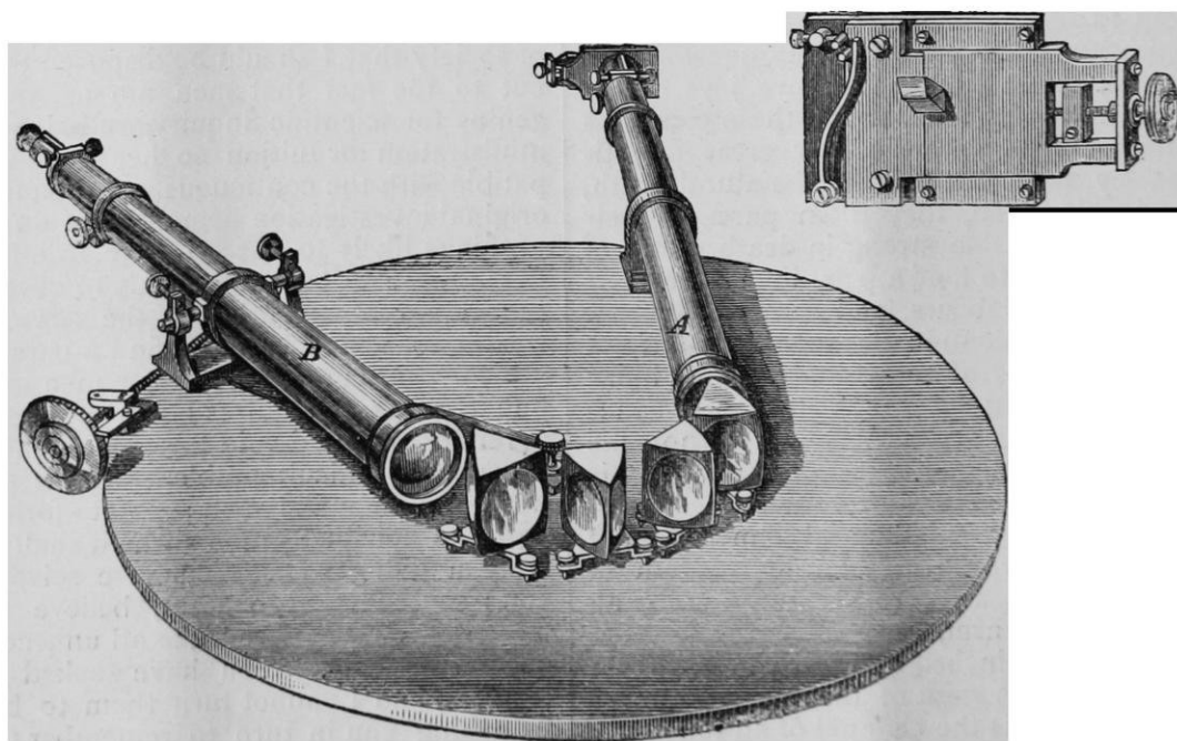
FIG. 14.—Steinheil's form of four-prism spectroscope; arrangement of slit shown separately.
