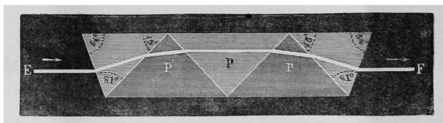
FIG. 18.—Direct-vision prism with five prisms.
