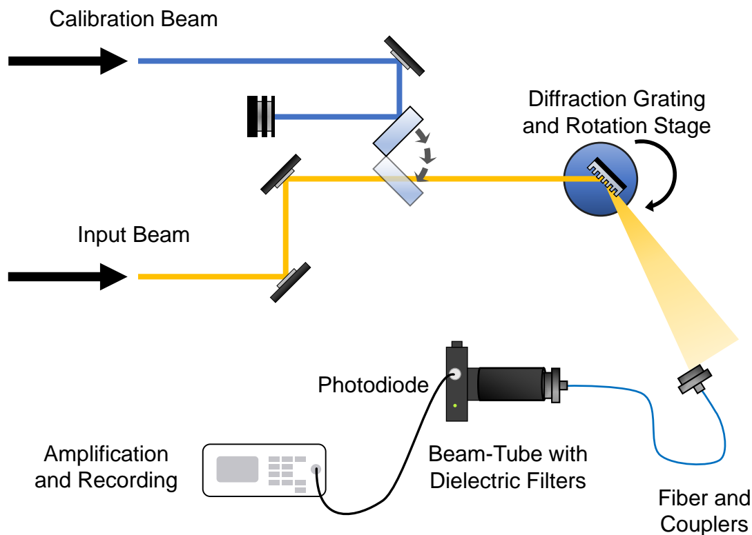
Figure 7.6: The Spectrometer
