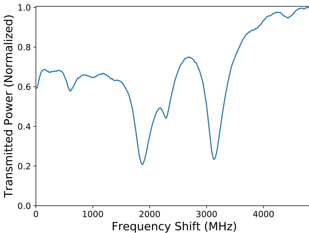
Figure 8.8: Microsphere Resonances
