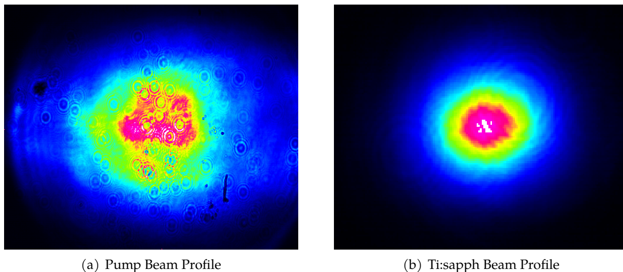
Figure 7.3: Beam Profiles
