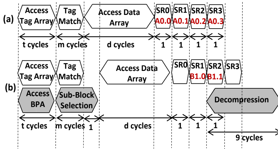
Figure 4-8: (a) Timing of a conventional cache and (b) DCC.
