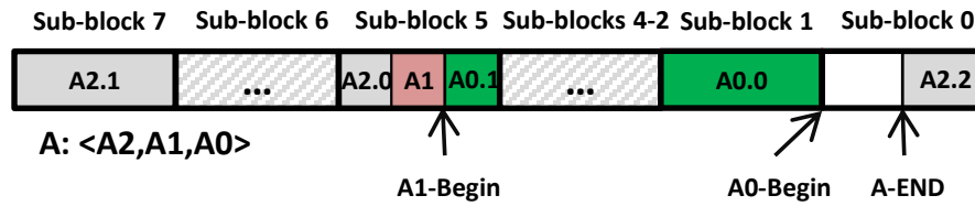
Figure 4-5: Co-DCC co-compaction
