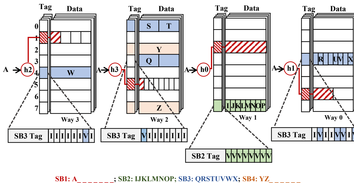
Figure 5-2: Skewed Compressed Cache.
