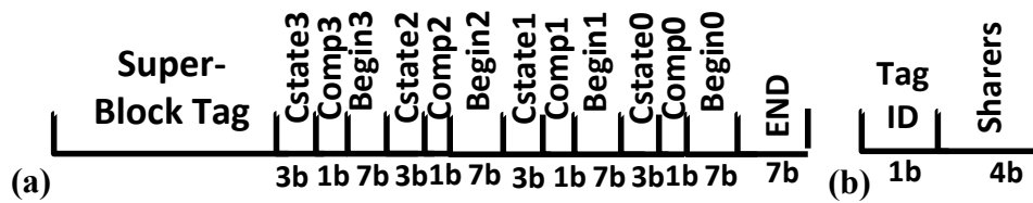
Figure 4-6: (a) One Co-DCC tag entry (b) One Co-DCC BPE.
