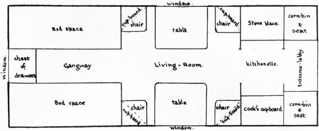
FLOOR PLAN OF CARAVAN.
