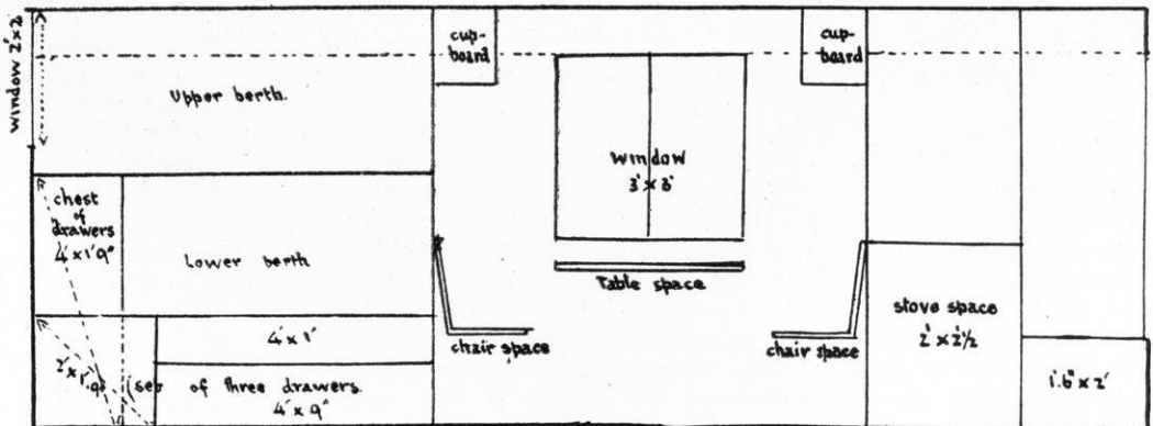
DETAIL PLAN OF CARAVAN, WITH GOOD PLACING OF CONVENIENCES.
