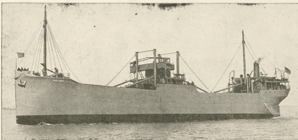
3400 D. W. T. Ocean-going Steamer, "Lake Linden," length overall, 261-0, moulded beam, 43 6, depth, 23-0
