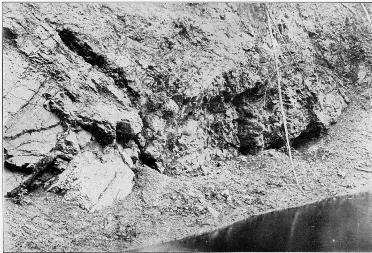
Fault Breccia in the Traps. Middle river contact of Traps and Lake Superior Sandstone.
