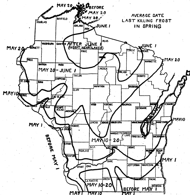
FIG. 3. LAST KILLING SPRING FROST.
