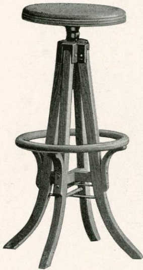
No. 200 Screw Stool Oak, Office Color, Rubbed Height 33 inches Seat 14 inches wide, 14 inches deep, 1½ inches thick K. D.
