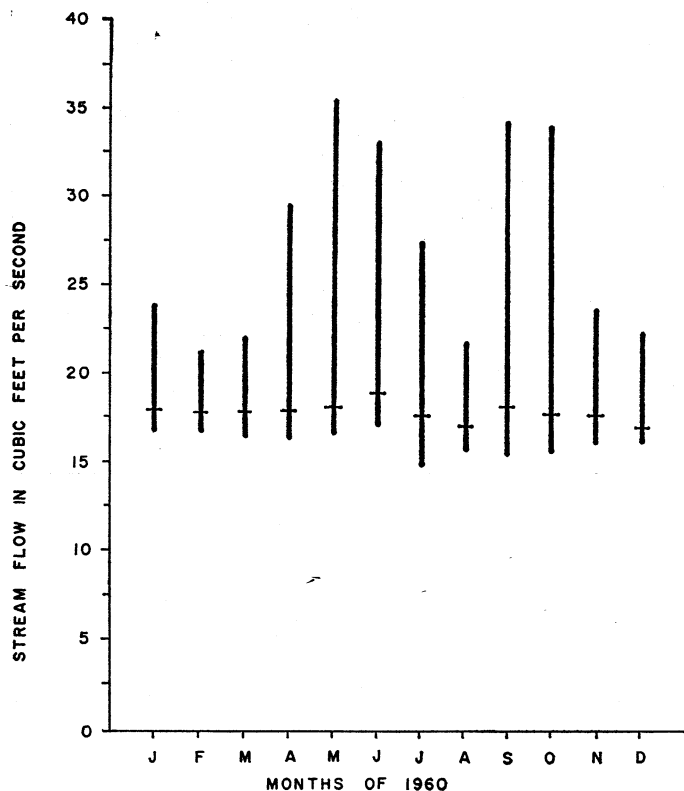
Figure 3. Monthly range and monthly mean streamflow of Lawrence Creek at the section C recorder site during 1960. Monthly means indicated by the cross-bars are averages of daily means for the month.
