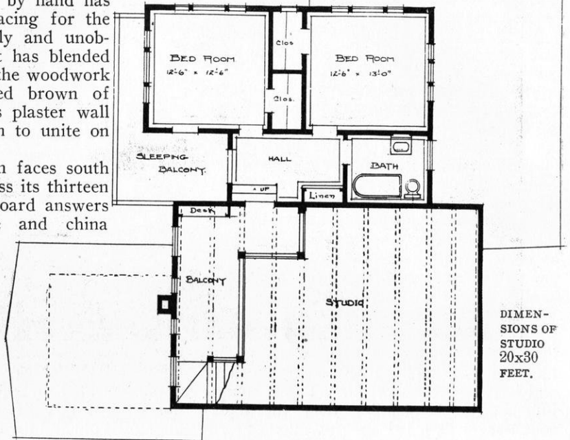
THE SECOND FLOOR PLAN OF THE HOUSE BUILT AROUND A STUDIO.
