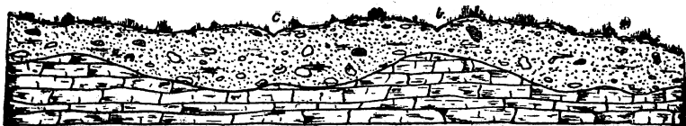
FIG. 3.—Diagrammatic section showing thick drift over rock.
