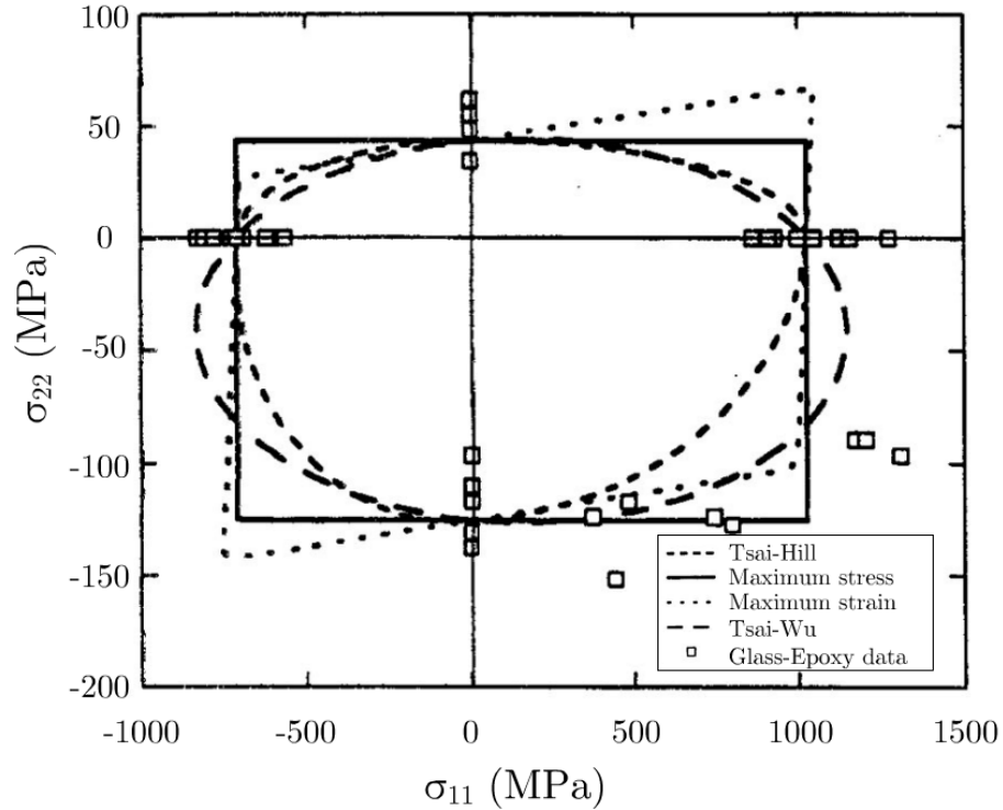
Figure 1.6: Comparison of different failure criteria. [31]
