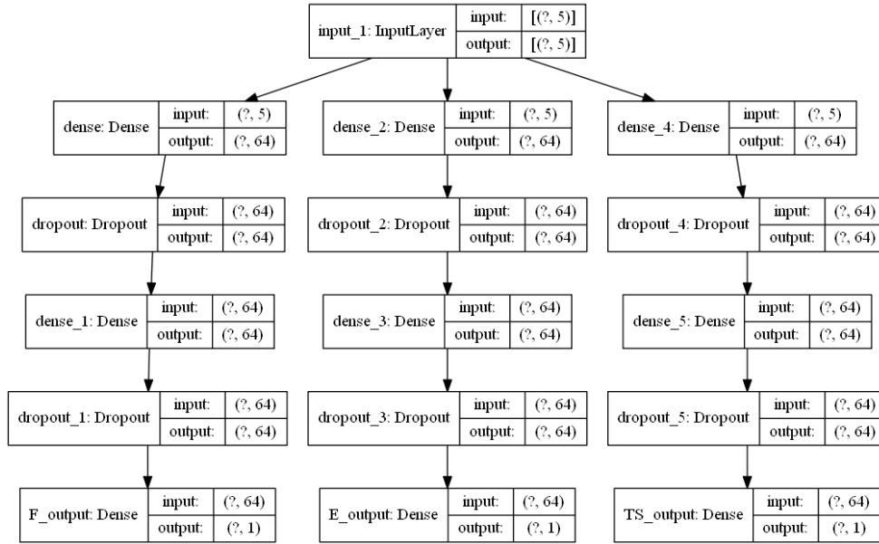
Figure 4.9: Preliminary architecture for the NN
