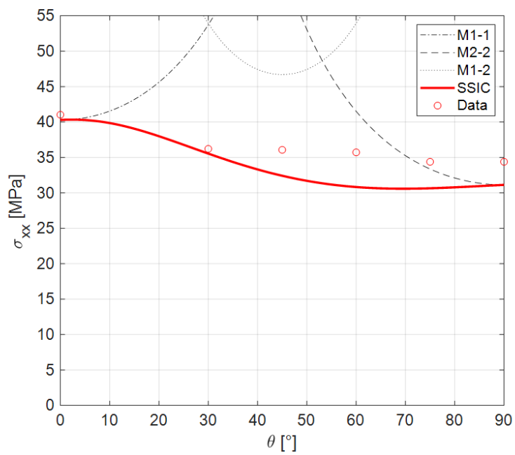
(b) Comparison of data and failure prediction using various FC
