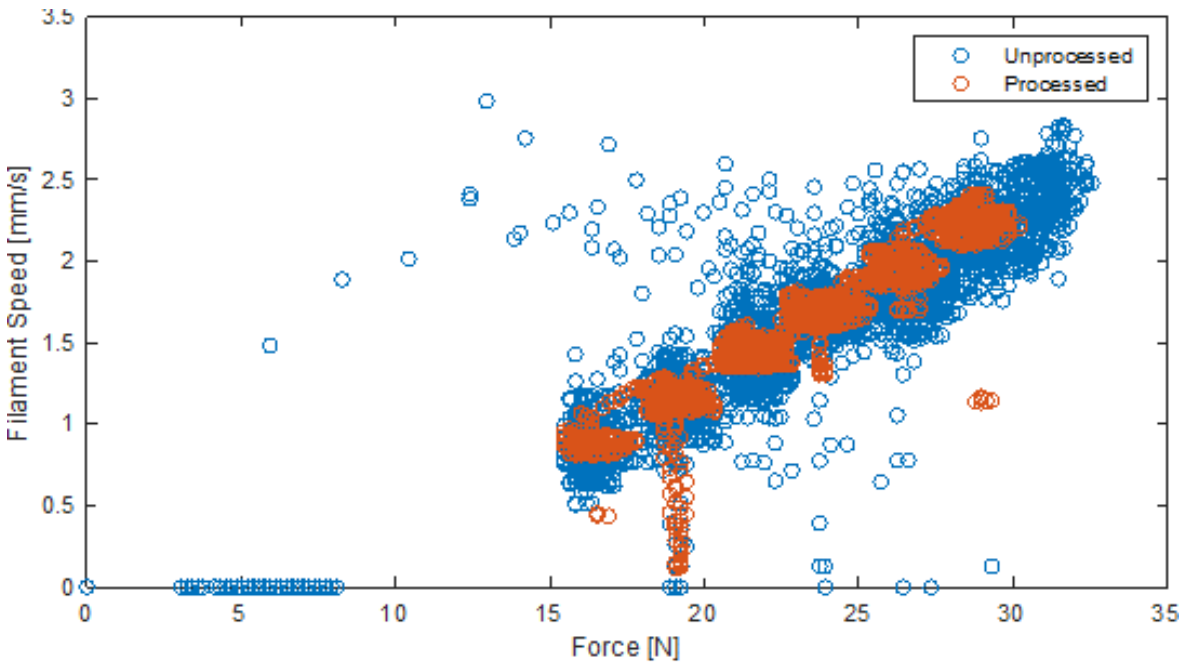
Figure 3.8: Comparison of processed and unprocessed filament speed vs. force within the nozzle of an FFF printer. PLA printed at 230°C.
