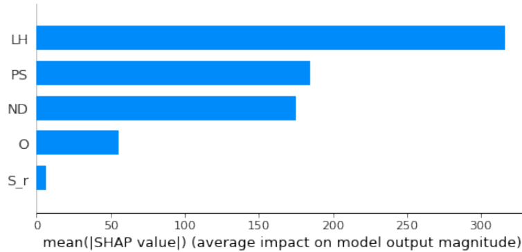
Figure 4.12: Mean Shapley values for Force output
