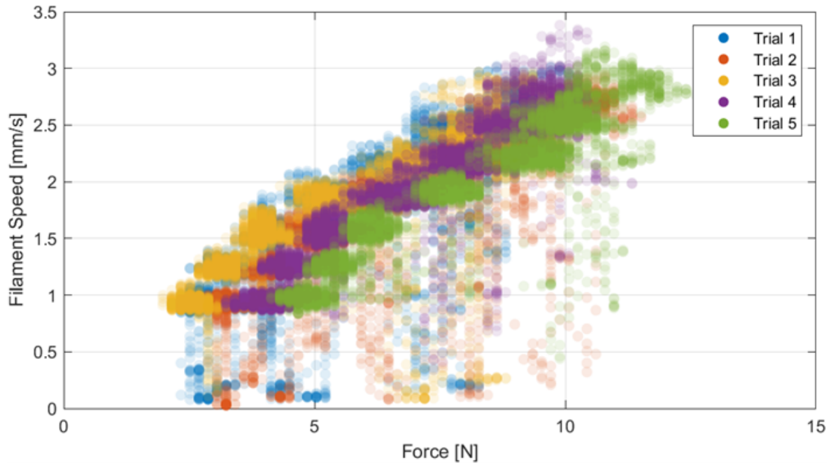
Figure 3.10: Alpha plot for 5 trials of ABS printed at 245°C.
