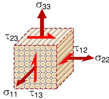
Figure 1.7: Different load directions in an anisotropic material
