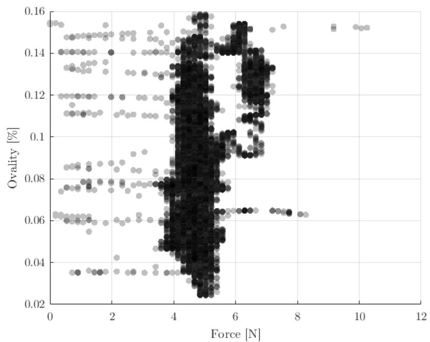
(a) Effect of ovality on measured filament force
