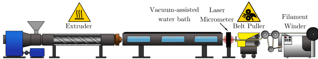
Figure 3.3: Extrusion line used to produce ABS filament
