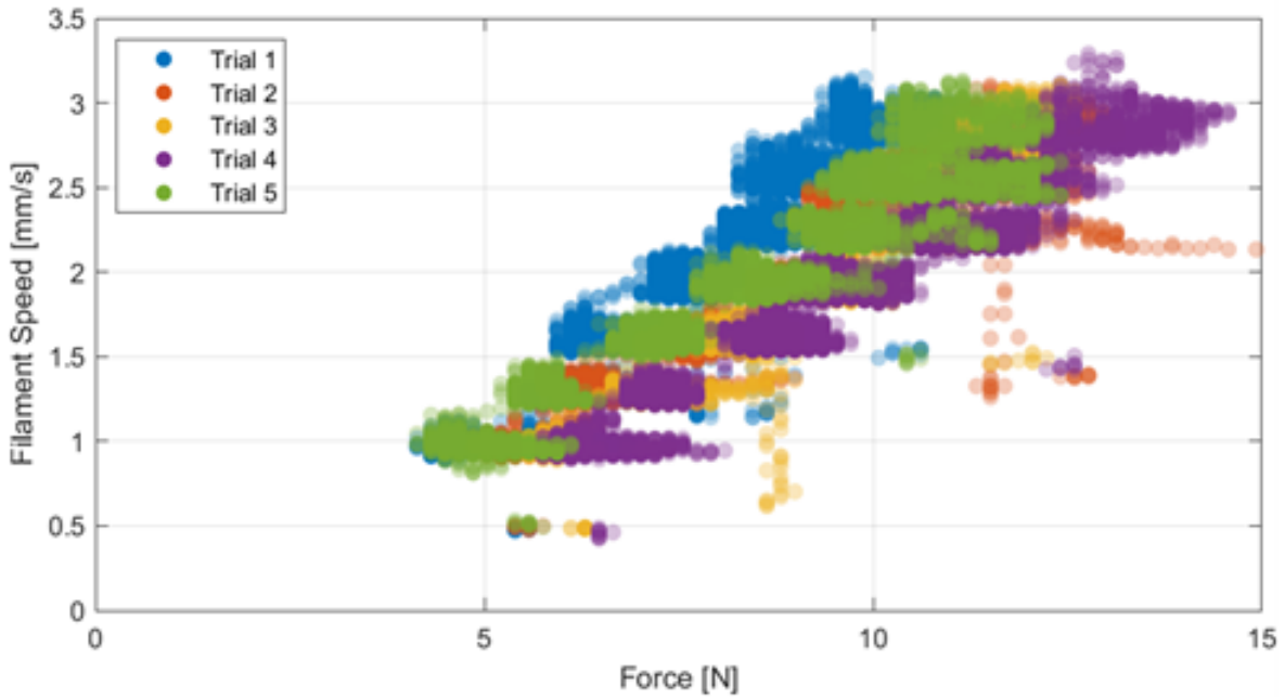
Figure 3.11: Alpha plot for 5 trials of PLA printed at 230°C.
