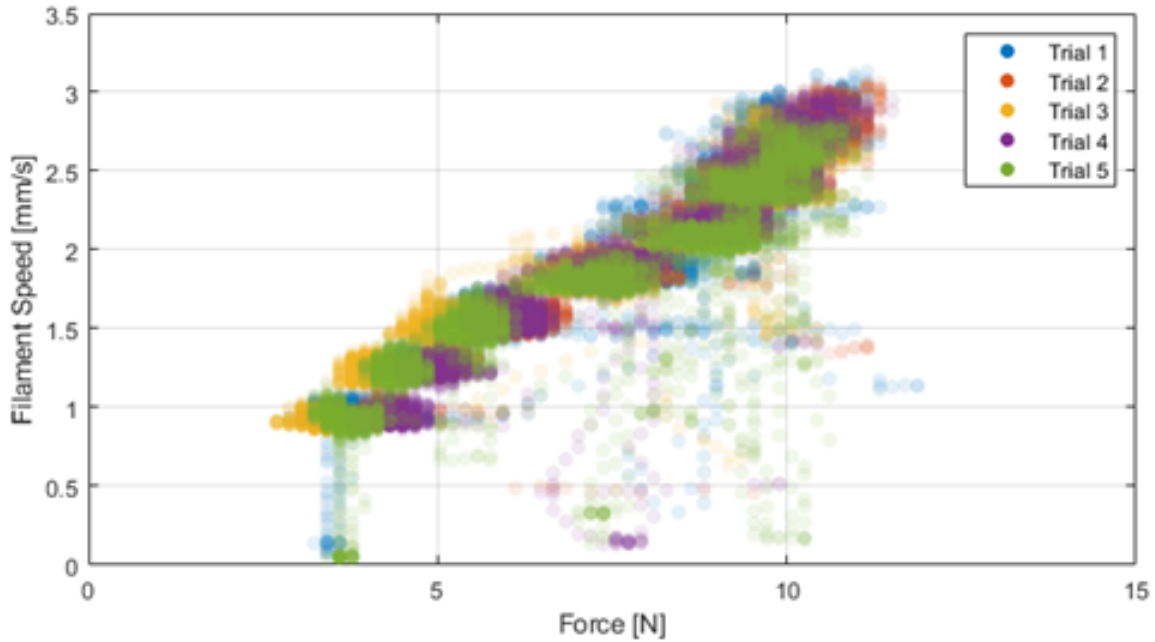
Figure 3.9: Alpha plot for 5 trials of ABS printed at 230°C.
