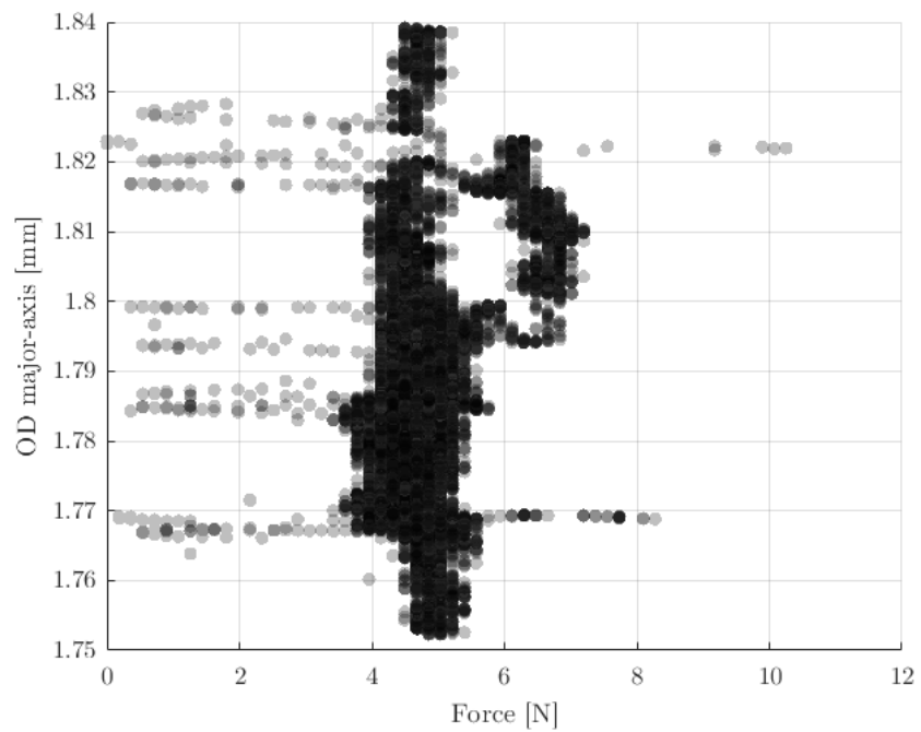
(b) Effect of diameter on measured filament force
