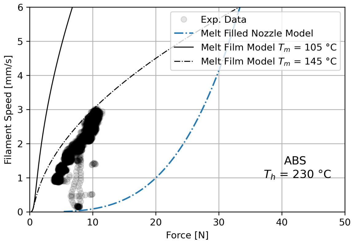
Figure 3.14: Comparison of experimental data for ABS printed at 230^\circ\text{C} with predictions stemming from various ME melting models.
