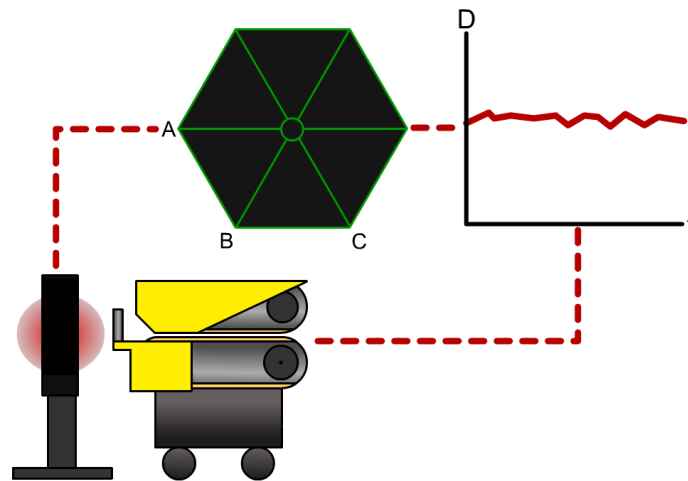
Figure 4.6: Filament geometry information, acquired through a laser micrometer
