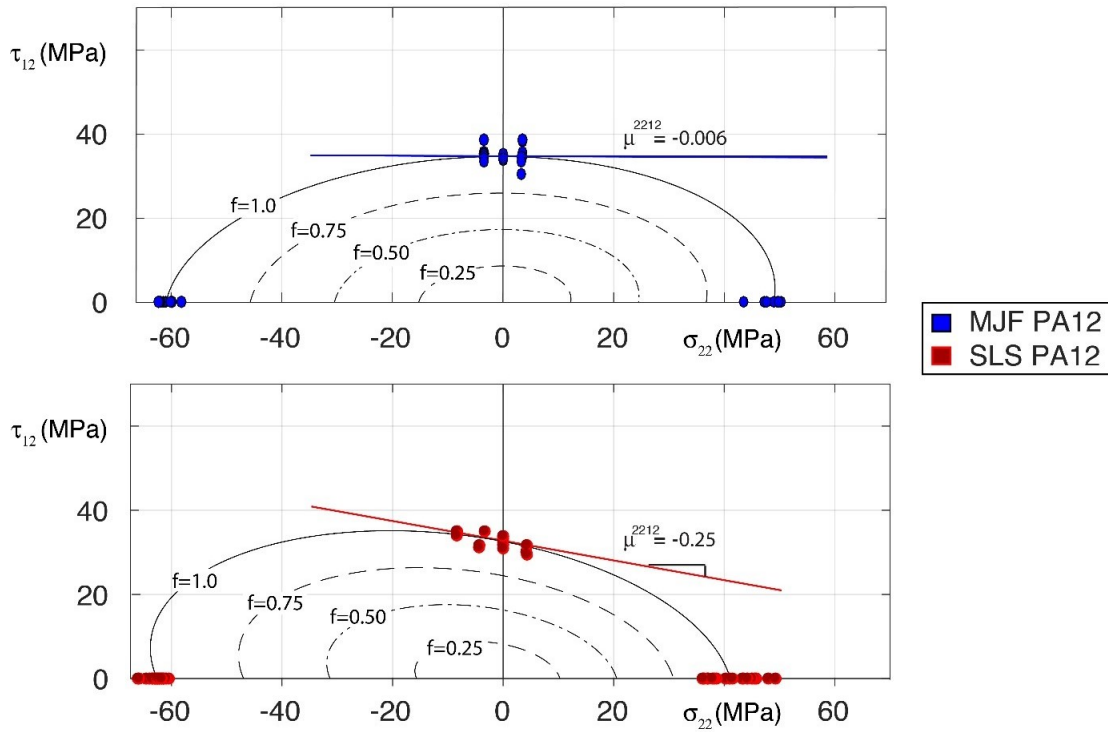
Figure 1.10: Comparison of the \sigma_{22} - \tau_{12} interaction for SLS and MJF PA12 parts [34]
