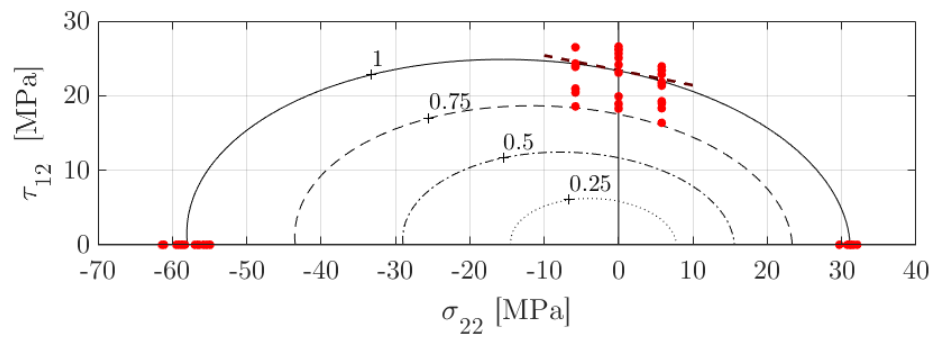
(b) failure envelope in the \sigma_{22} - \tau_{12} plane
