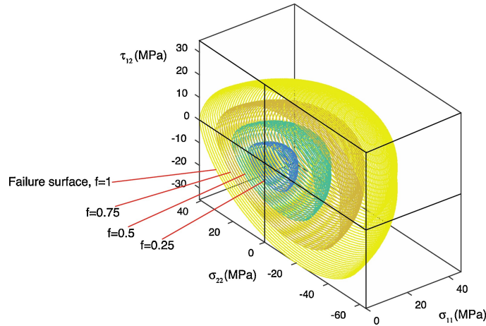
Figure 1.9: Failure surface for SLS developed through the SSIC [8]
