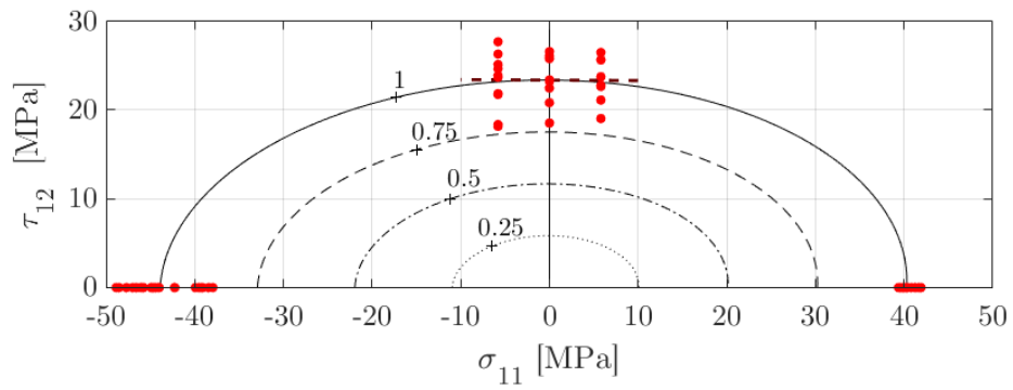
(a) failure envelope in the \sigma_{11} - \tau_{12} plane
