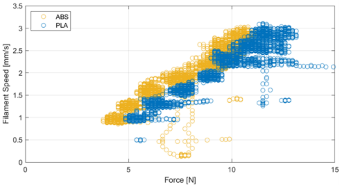
Figure 3.12: Comparison of PLA and ABS Force-velocity pairings at a printing temperature of 230°C
