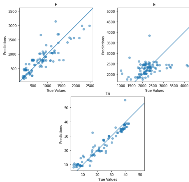
Figure 4.11: Comparison of predictions and true outputs using the validation set
