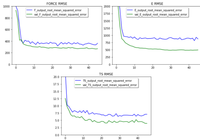
Figure 4.10: Learning curves for filament force (F), tensile modulus (E), and tensile strength (TS) using the RMSE metric
