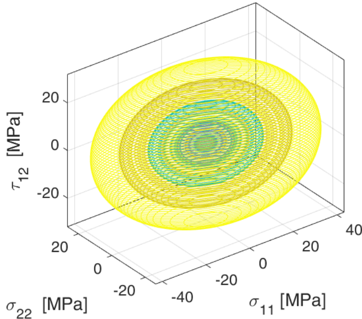
Figure 4.14: Conservative Failure Surface predicted through the NN
