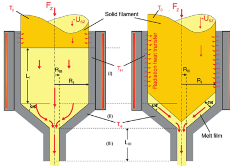
Figure 3.1: Bellini model (left) and Osswald, Puentes, Kattinger model (right) [43].
