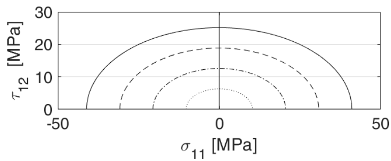
(b) Predicted failure envelope projection in the \sigma_{11} - \tau_{12} plane
