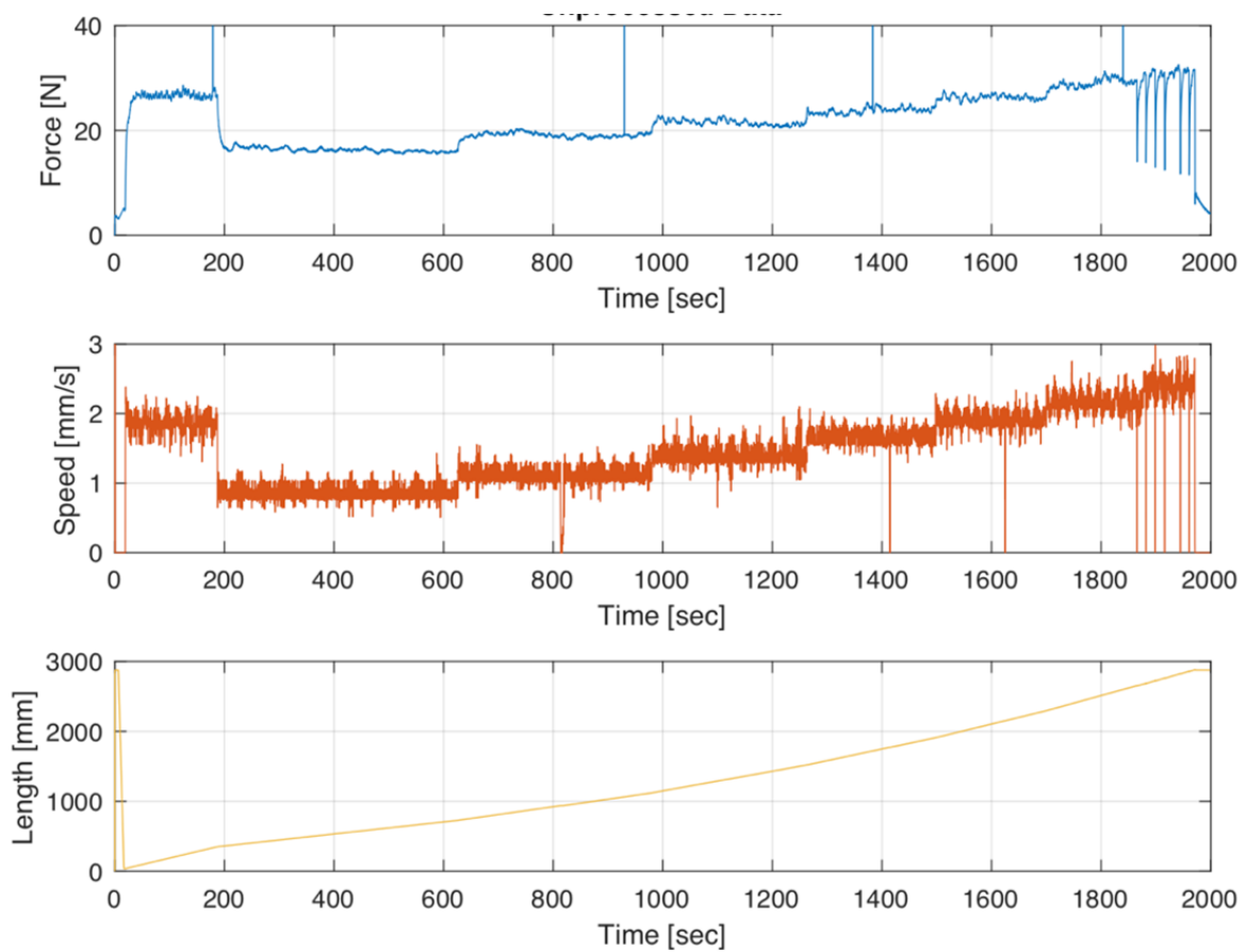
Figure 3.6: Raw signal data length (bottom), derived speed (middle), and force (top).
