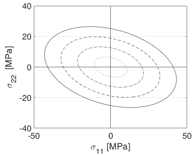
(a) Predicted failure envelope projection in the \sigma_{11} - \sigma_{22} plane
