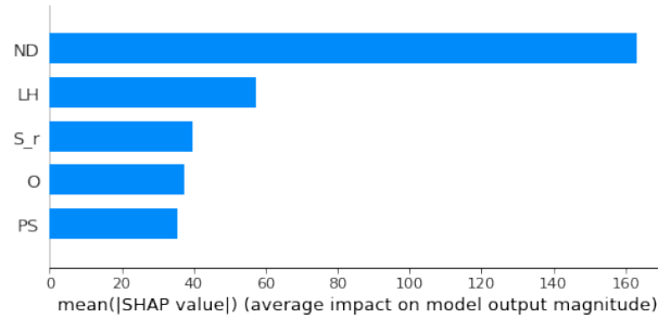
(a) Mean Shapley values for Modulus output
