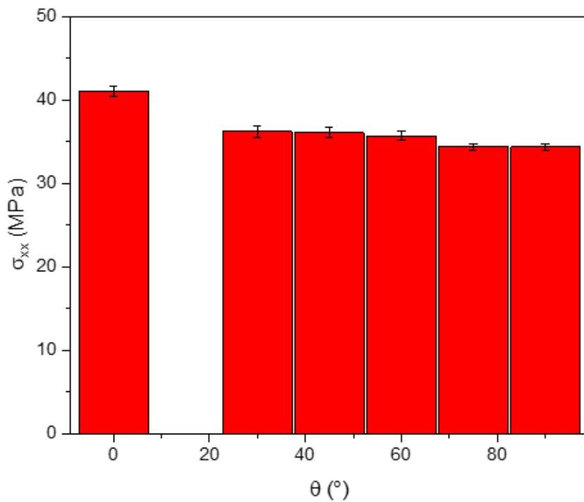
Figure 2.2: Experimental results from tensile tests
