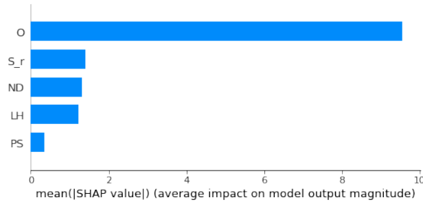
(b) Mean Shapley values for Tensile Strength output
