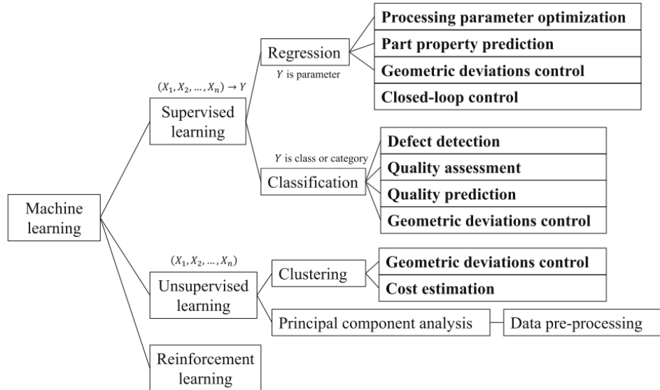
Figure 1.14: Taxonomy of ML applications in AM [15]
