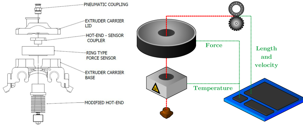
Figure 3.2: Assembly shown on the left. Schematic of sensor placement on the right.
