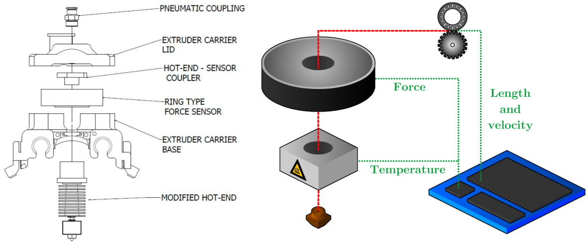
Figure 4.4: Schematic of modified ME printer with sensors
