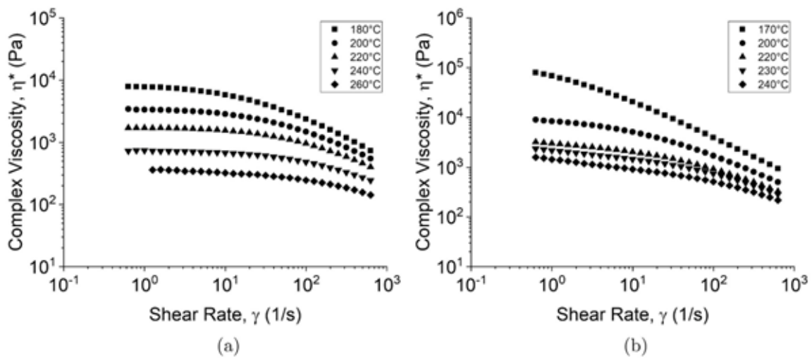
Figure 3.4: Shear rate dependency for a) PLA and b) ABS
