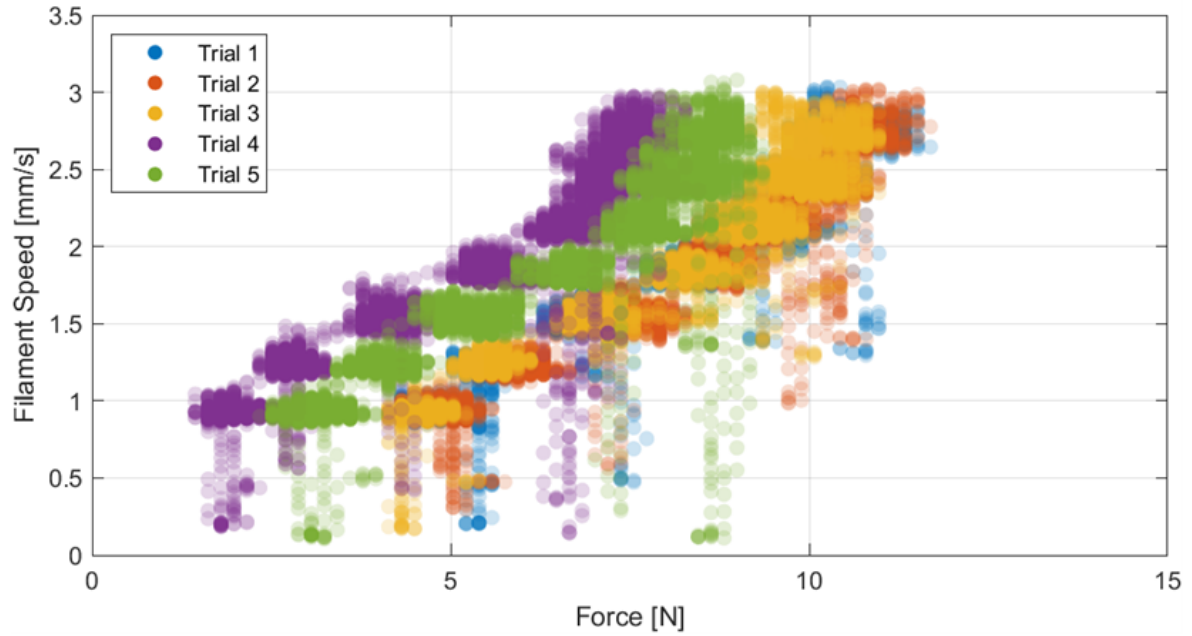
Figure 3.13: Alpha plot for 5 trials of PLA printed at 245°C.
