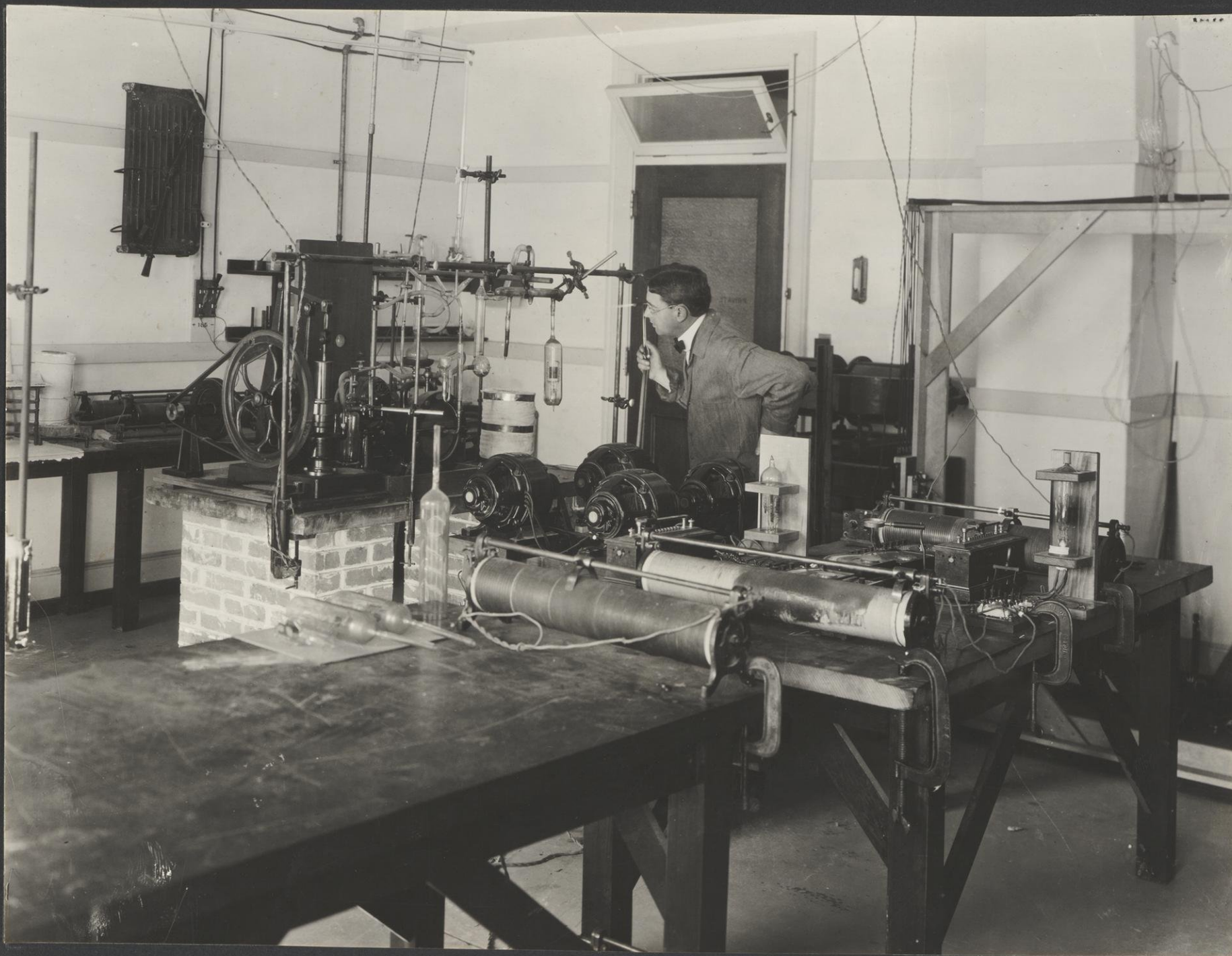
RADIO ELECTRICIANS MANUFACTURE OF VACUUM TUBES FOR RADIO TELEPHONY
