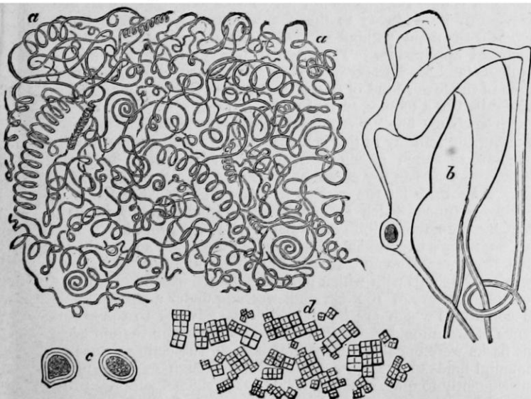
FIG. 13.—Spirally Twisted Fibre Organism.
