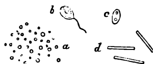
FIG. 16.—Tailed Monad and Torula Cell from a Turnip Solution which had been exposed to a temperature of 146^{\circ} — 153^{\circ}\text{C} . for four hours.
