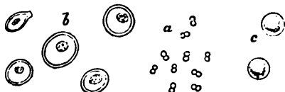
FIG. 18.—Fungus-spores found in a Carbonate of Ammonia and Phosphate of Soda Solution which had been exposed to a temperature varying from 146° to 153° C. for four hours.
