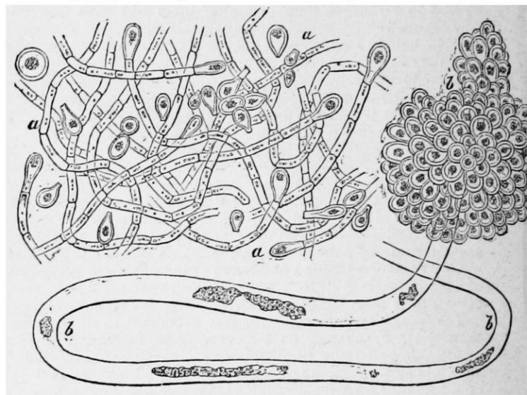
FIG. 17.—Fungus obtained from a solution of Tartrate of Ammonia and Phosphate of Soda which had been exposed to a temperature varying between 146^{\circ} and 153^{\circ} C. for four hours.
