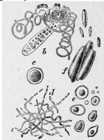
FIG. 11.—Spiral and Confervoid-looking Filaments, with Fungus-spores and Crystals, from a Tartrate of Ammonia Solution.
