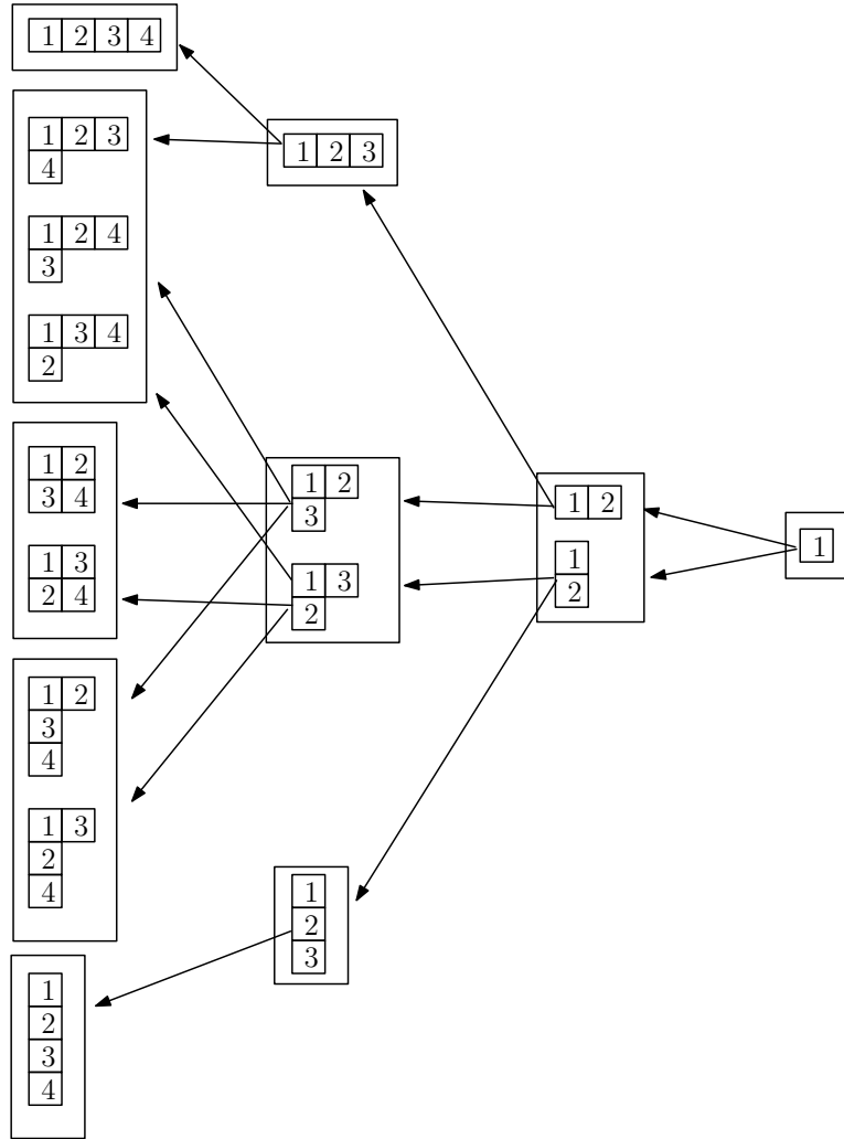
Figure 2.2: The extended Brattelli diagram for \mathbb{S}_4 .
