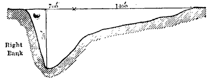
FIG. 3.—Ordinary Section—no irrigation canals.
