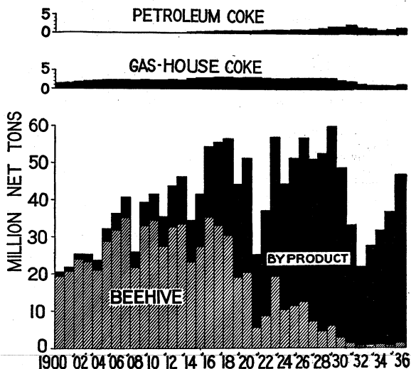
FIGURE 58.—Production of petroleum coke, gas-house coke, and beehive and byproduct coke in the United States, 1900-1936. No figures on production of petroleum coke are available before 1914, when the production was 213,777 tons.
