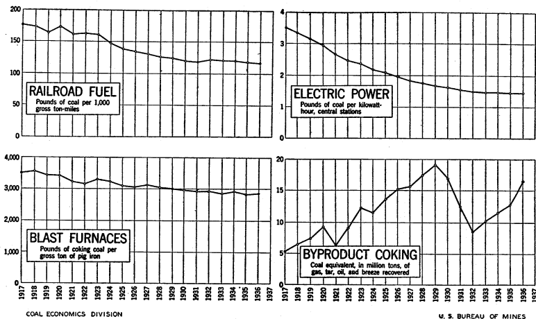
FIGURE 53.—Trends in fuel efficiency in the United States, 1917-36.
