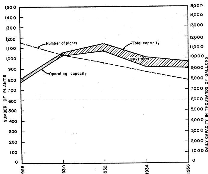
FIGURE 76.—Number and capacity of natural-gasoline plants on January 1, 1928, 1930, 1932, 1934, and 1936.
