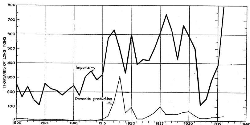
FIGURE 36.—Imports and domestic production of manganese ore, 1900-1936. Statistics on imports shown in the graph represent "general imports" for the period 1900-1933; beginning with 1934 data classified as "general imports" were not available, and the figures plotted for 1934, 1935, and 1936 represent imports for consumption adjusted for changes in stocks in bonded warehouses and are closely comparable with the record for earlier years.
