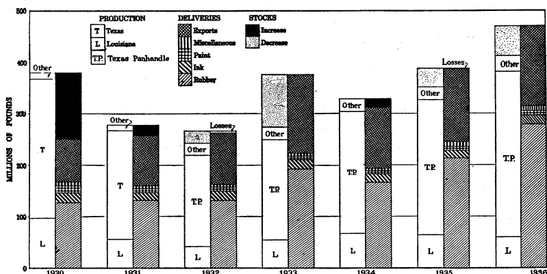
FIGURE 80.—Production and consumption of carbon black, 1930-36.
