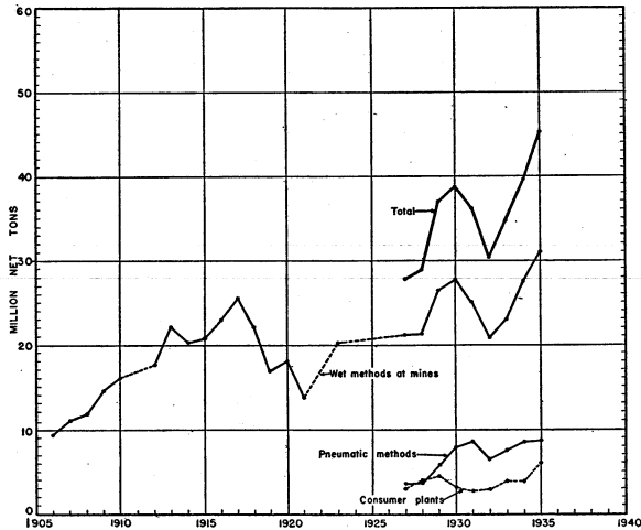
FIGURE 52.—Tonnage of bituminous coal mechanically cleaned, 1906-35.
