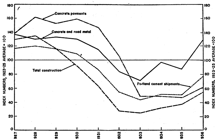
FIGURE 84.—Sales of concrete and road metal (crushed stone) compared with total construction, portland-cement shipments, and contracts for concrete pavements, 1927-36. Data are plotted as index numbers with the 1923-25 average as 100. Figures on cement and stone compiled by the Bureau of Mines, on concrete pavements by the Portland Cement Association, and on construction contracts by the F. W. Dodge Corporation.
