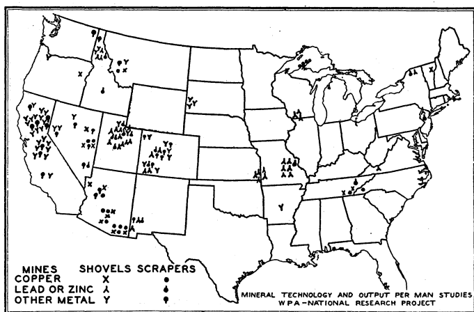
FIGURE 24.—Localities in which scraper and shovel loaders have been introduced underground in nonferrous metal mines.
