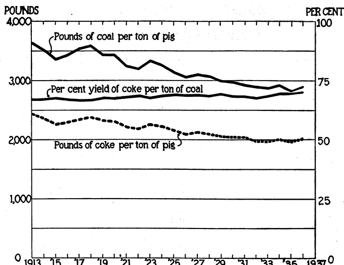
FIGURE 61.—Gross value of the several byproducts per ton of byproduct coke produced, 1913-36.
