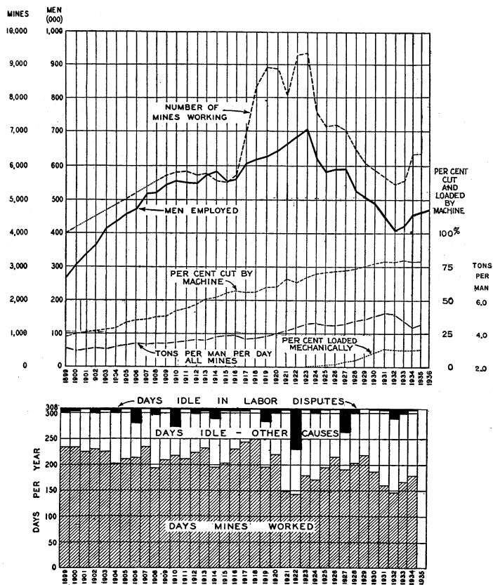
FIGURE 51.—Trends of employment, working time, mechanization, and output per man at bituminous coal mines, 1899-1936.
