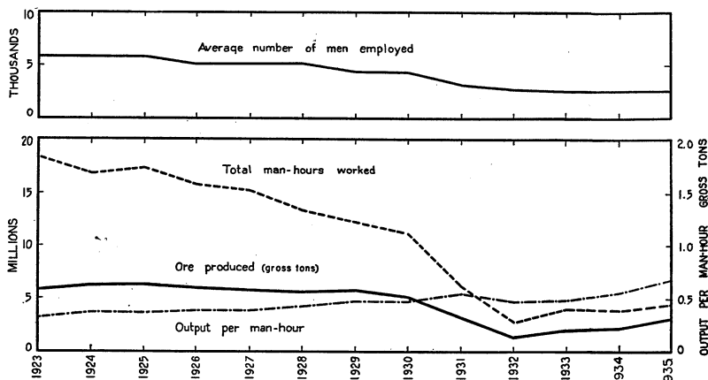
FIGURE 35.—Trends in production, man-hours worked, output per man-hour, and number of men employed at iron-ore mines in Jefferson County, Ala., 1923-35.
