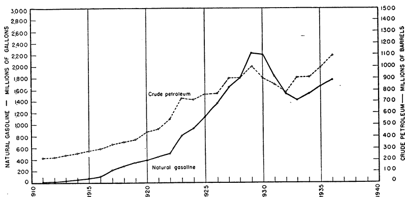
FIGURE 78.—Annual production of natural gasoline and crude petroleum, 1911-36.
