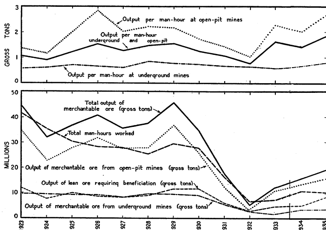
FIGURE 34.—Trends in output of merchantable iron ore per man-hour at open-pit and underground mines in Minnesota compared with production of merchantable and lean ore, and total man-hours worked, 1923-35.
