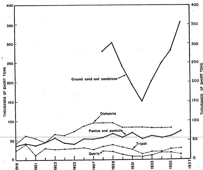
FIGURE 100.—Trends in production of diatomite, tripoli, pumice and pumicite, quartz, and ground sand and sandstone, 1919-36.
