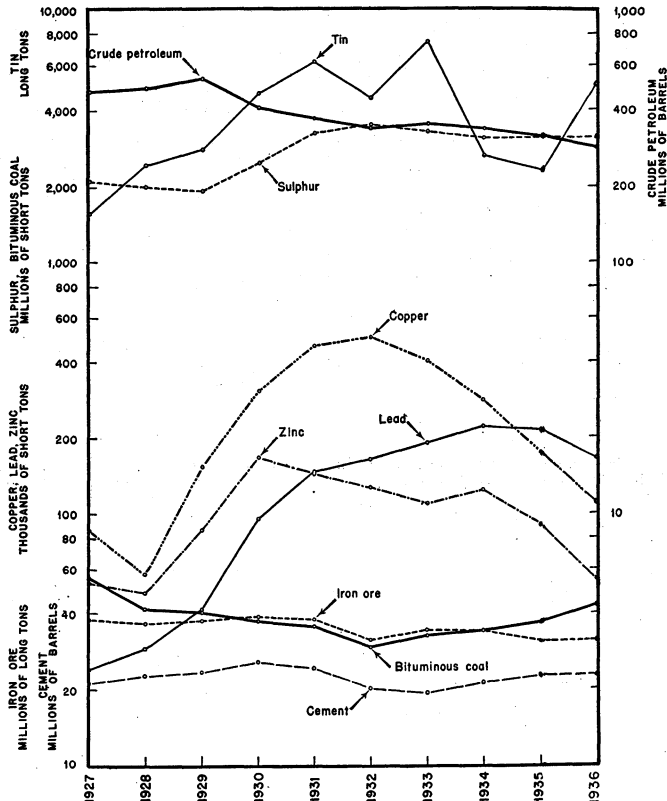
FIGURE 9.—Trends in mineral stocks in the United States, 1927-36.
