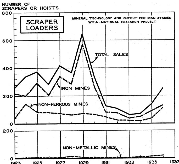
FIGURE 21.—Shipments of scraper loaders for use underground in metal or nonmetal mines, 1923-36. Note that the figures represent number of units only without regard to capacity. Were it possible to allow for the large increase in the size of machines during this period, the sales in recent years would look proportionately larger. Based upon detailed reports from eight manufacturers, with an estimate for one company not heard from when the books were closed.
