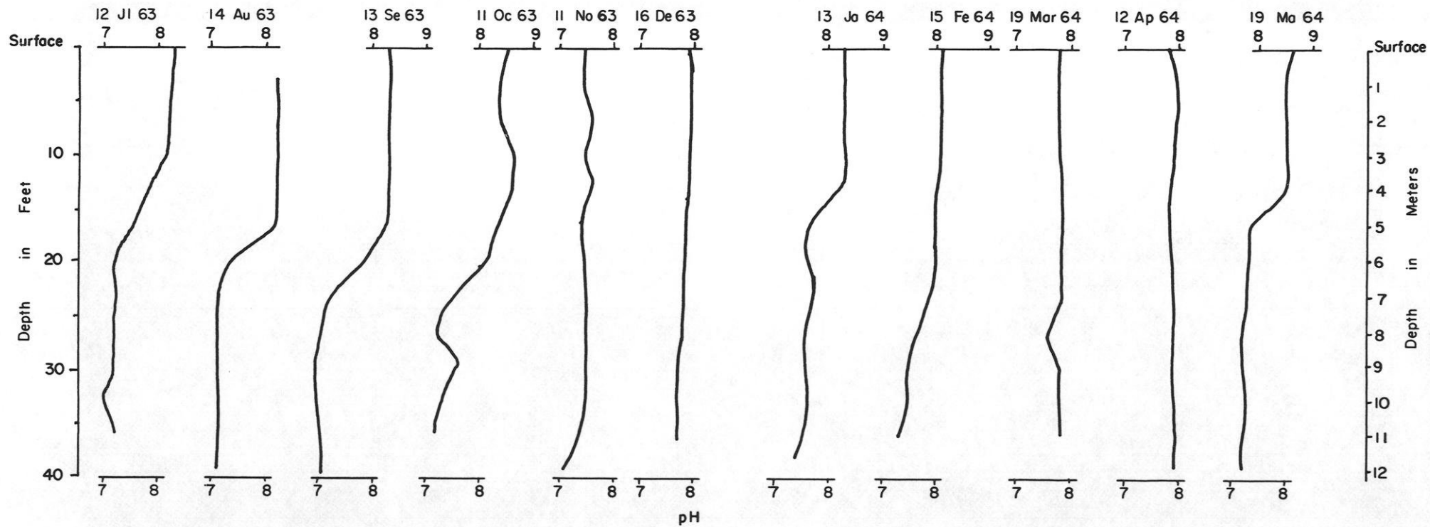
Figure II. pH Profiles.
