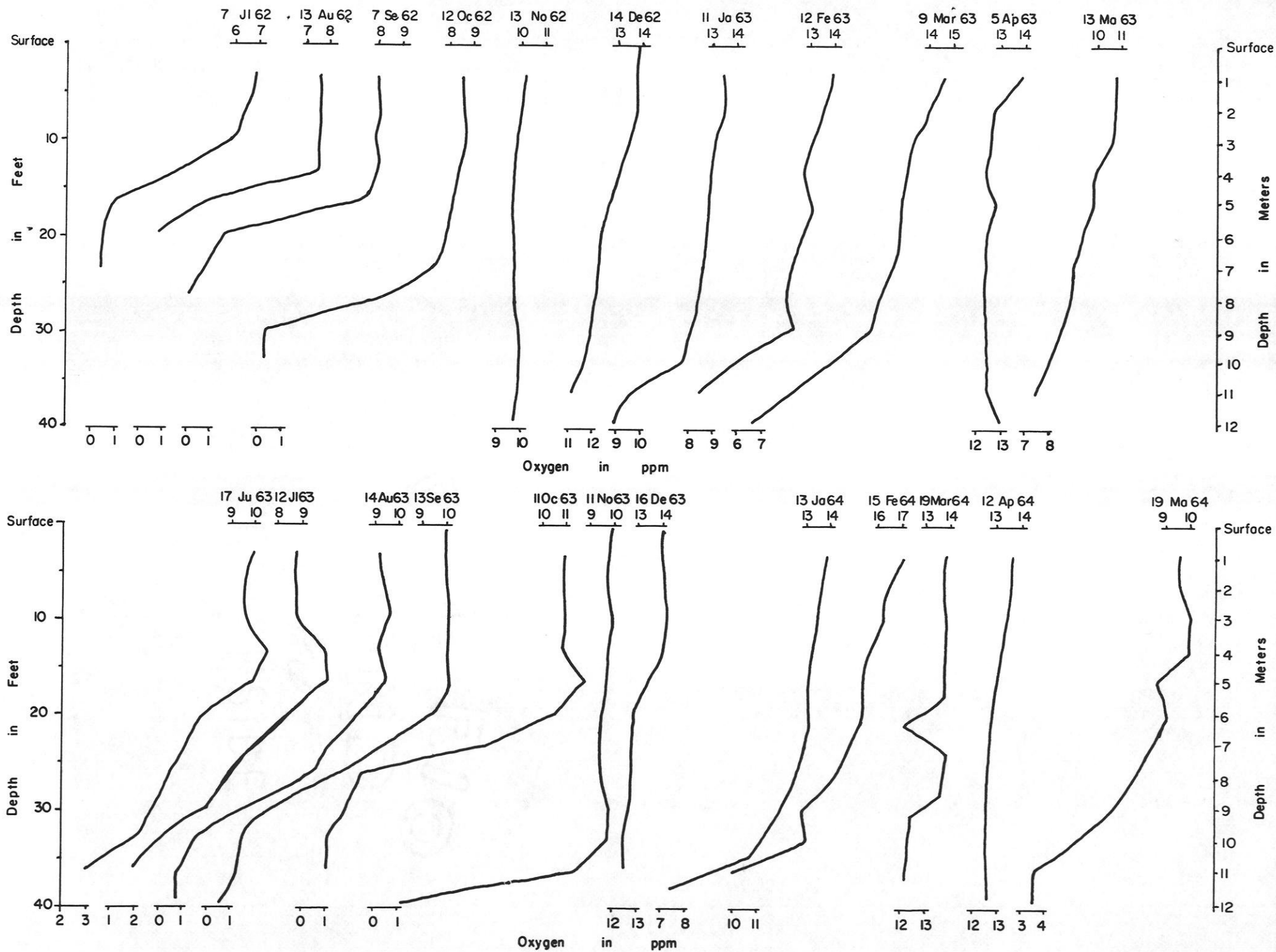
Figure 7. Oxygen Profiles.
