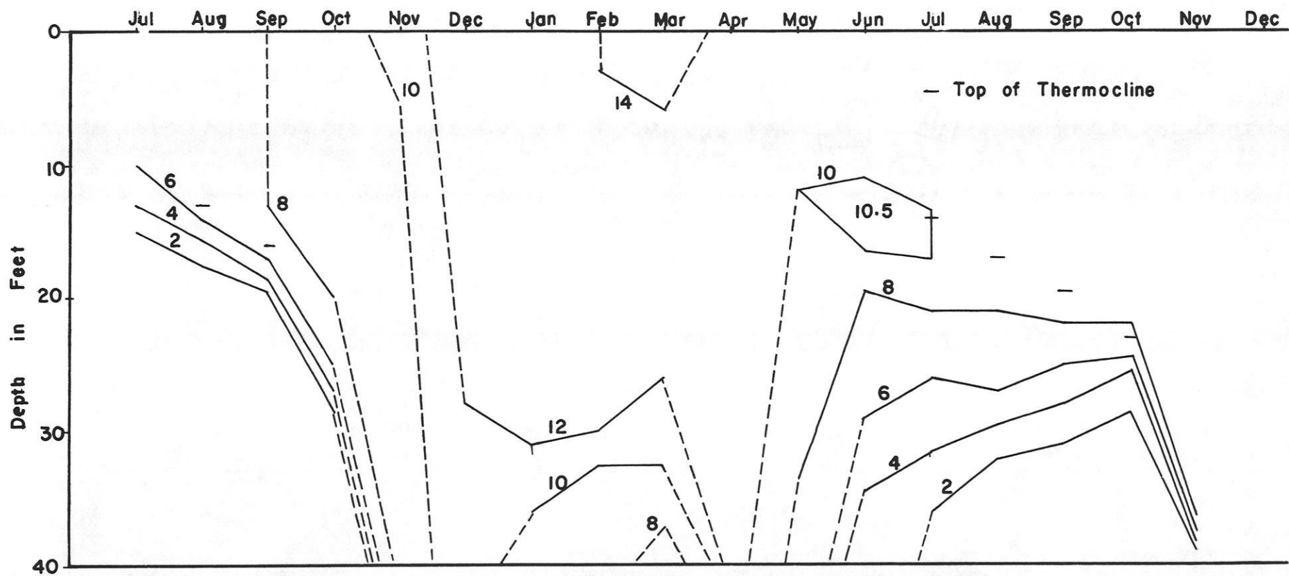
Figure 8. Lines of equal Oxygen concentration July 1962 - November 1963
