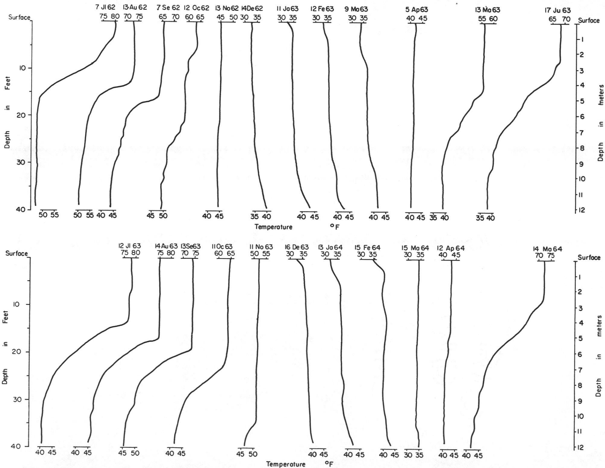
Figure 5. Temperature Profiles.
