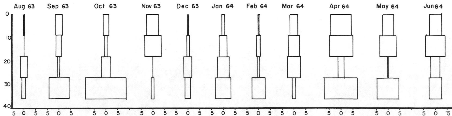
Figure 13. Copepod Distribution .
