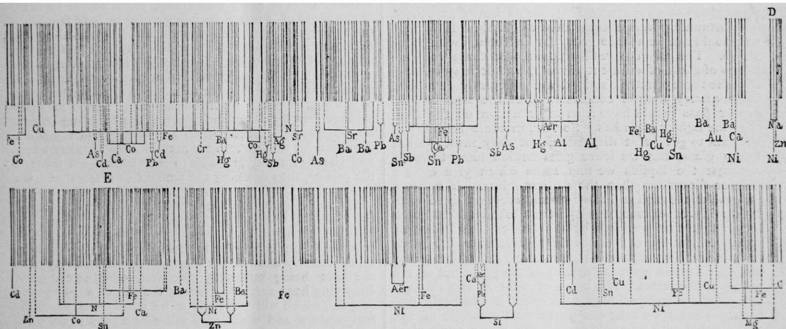
FIG. 12.—Upper diagram, Spectrum near D: Lower diagram, Spectrum near E.
