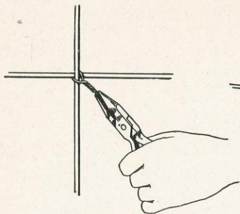
TO TIE TWO WIRES DIAGONALLY WITH USE OF TIE WIRE
