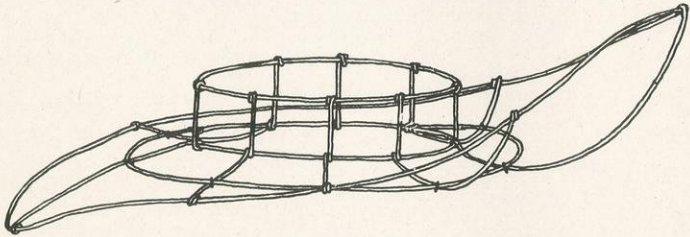
ROLLING WIRE BRIM. EIGHT SPOKES MORE MAY BE USED AND AS MANY CIRCLES AS WISHED, ACCORDING TO THE COVERING USED
