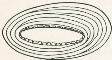
BRAID-COVERED BRIM SHOWING METHOD OF FILLING IN SHORT LENGTHS WHEN THE DIFFERENCE IN WIDTH OF THE TWO SIDES IS VERY GREAT
