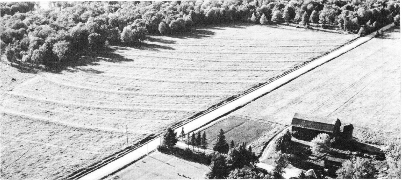
Figure 66 PARALLEL TERRACES
