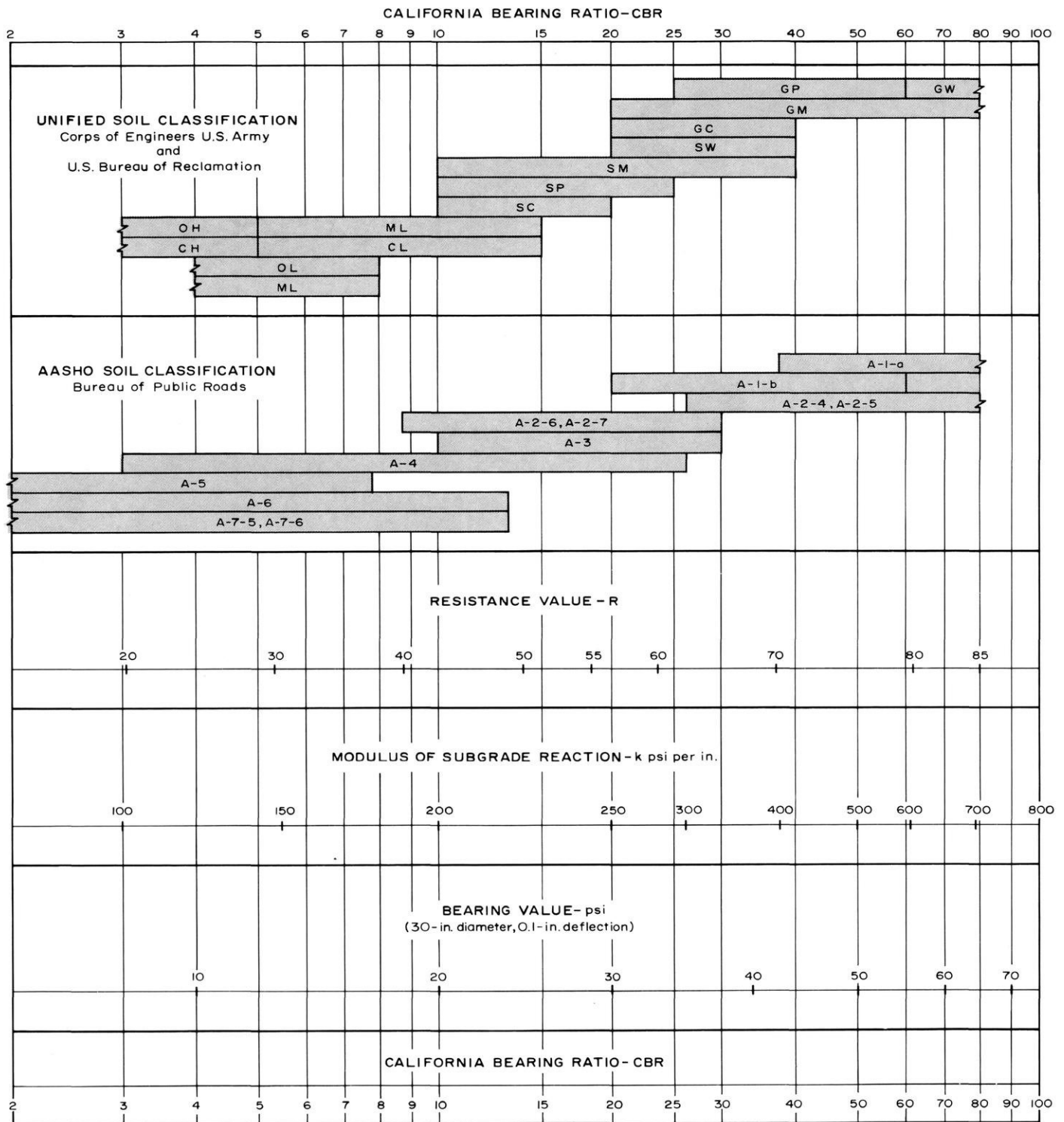
Figure 78 APPROXIMATE INTERRELATIONSHIPS OF SOIL CLASSIFICATIONS AND BEARING VALUES
