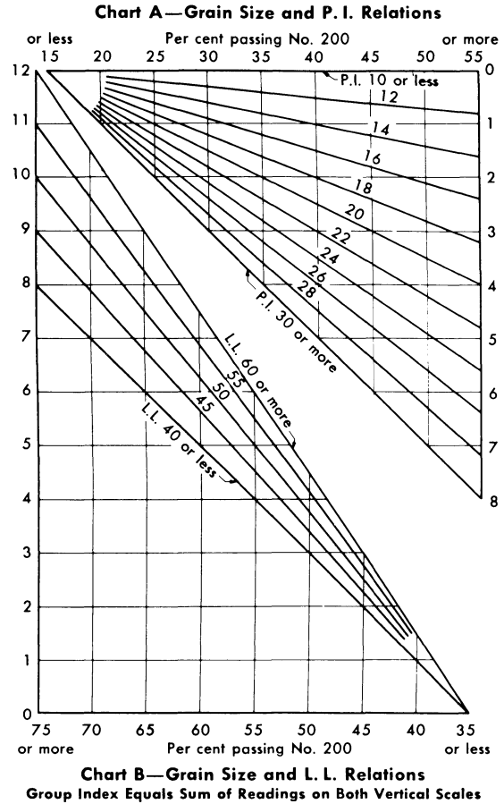
Figure 7 THE AASHO SOIL CLASSIFICATION SYSTEM
