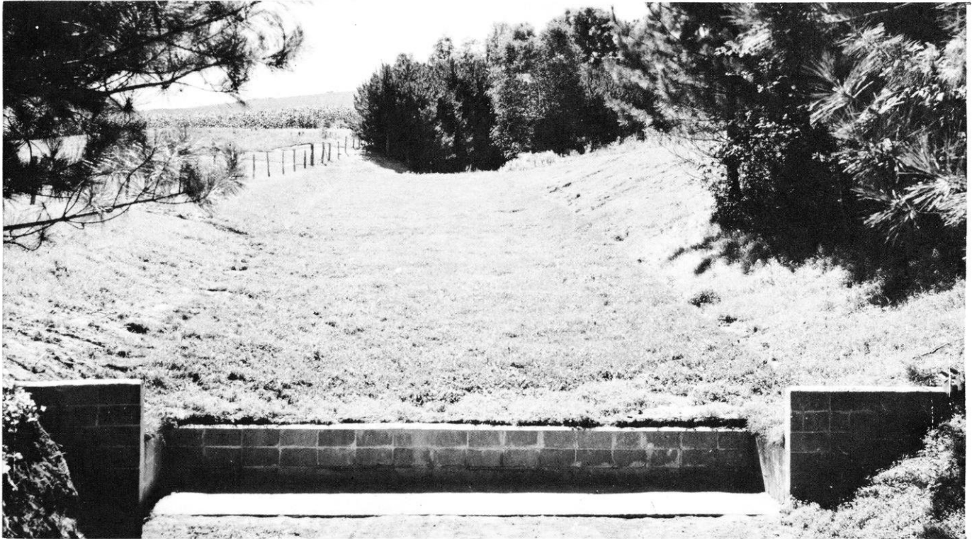
Figure 68 GRASSED WATERWAYS
