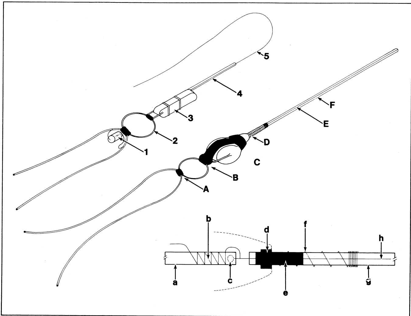
FIGURE 8. The transmitter described by Brander (1968) and the model used in this study are depicted for comparison. Brander transmitter: 1. battery; 2. harness incorporating battery leads; 3. component package; 4. plastic tubing; 5. whip antenna. Our transmitter: A. harness junction formed by square knot with cover of electrical tape; B. harness junction formed as described in Figure 2; C. transmitter package including battery encapsulated with dental acrylic; D. antenna protective system pictured in detail in Insert; E. gold-plated whip antenna; F. polyvinyl chloride tubing encasing entire antenna. Insert: a. poly-
