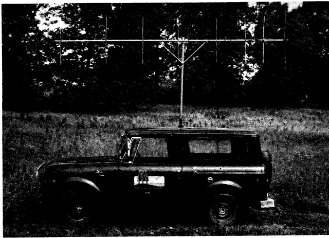
Directional antennas affixed to an internally rotated shaft
