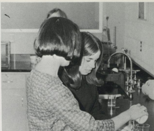
The two girls above are neutralizing an acid with a base to make a salt.
