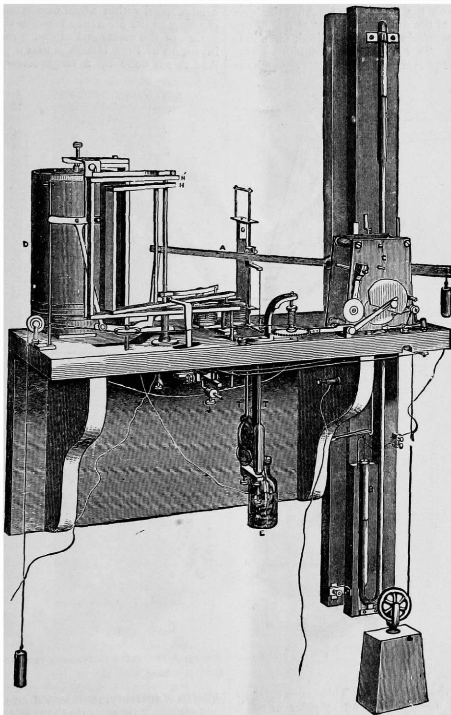
FIG. 8.—THE METEOROGRAPH
