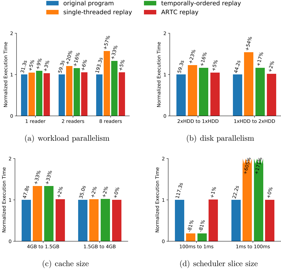
Figure 2.8: Microbenchmarks. Effect of feedback loops on accuracy. Labels on the original-program bars indicate running times for the original program on the target system. Labels on other bars indicate a percentage error relative to the original.
