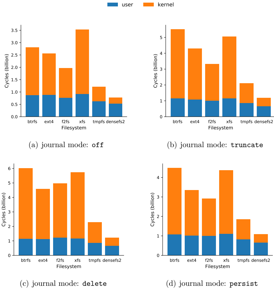
Figure 4.17: User- and kernel-mode CPU cycle counts for SQLite random-insert benchmark with the unix-dotfile vfs, C version.
