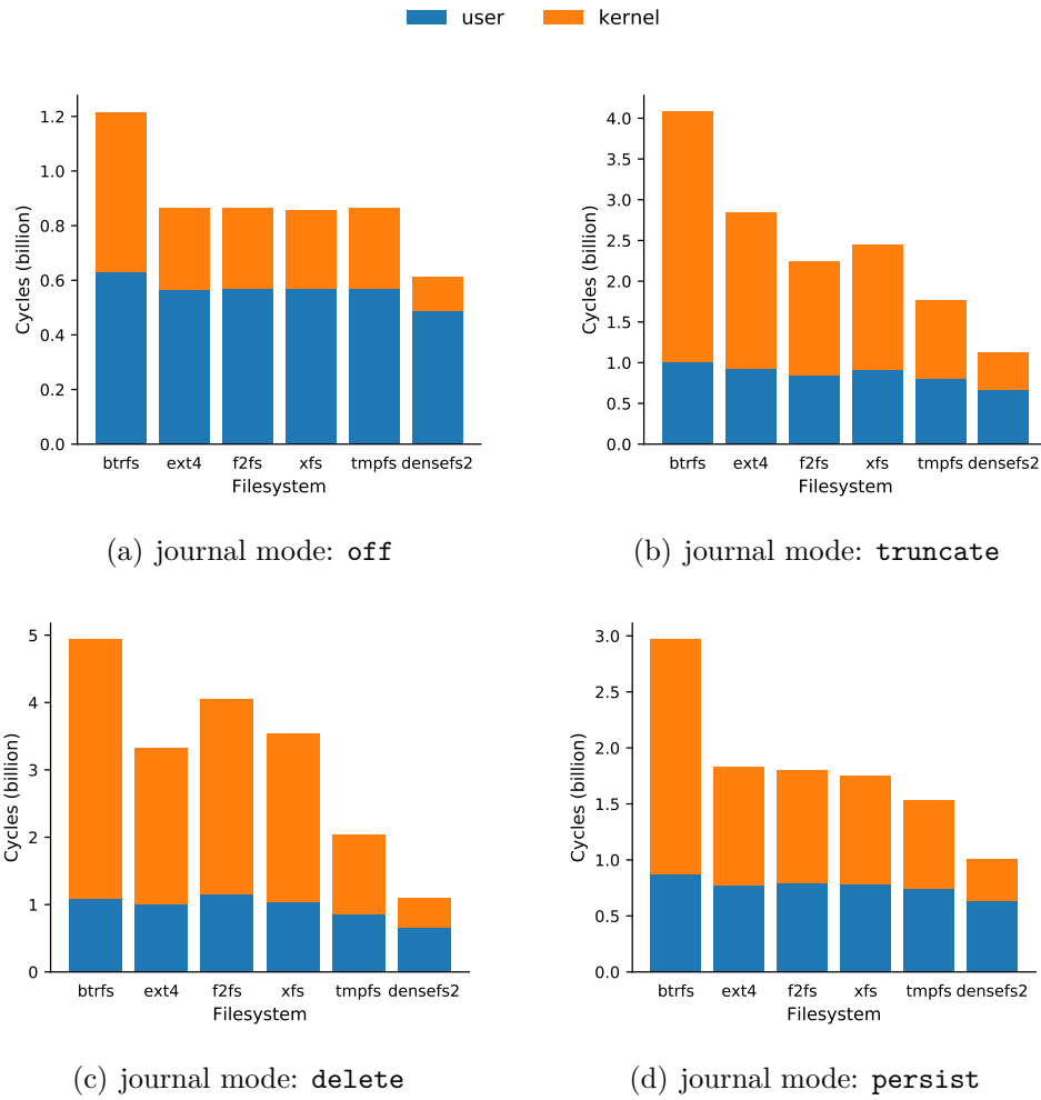
Figure 4.15: User- and kernel-mode CPU cycle counts for SQLite random-insert benchmark with the unix-none vfs, C version.
