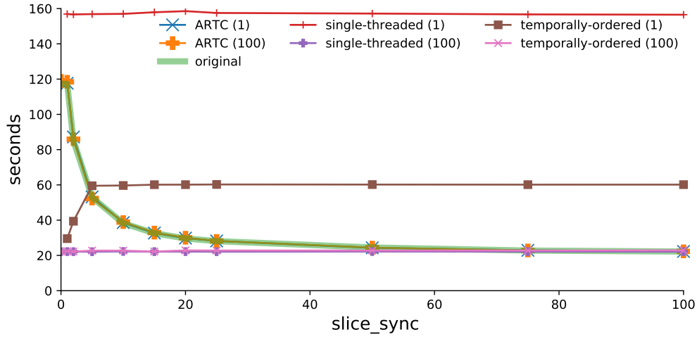
Figure 2.9: Varying anticipation. Throughput achieved by executions with varying slice_sync values. Performance is shown for the original program and three replays of two traces (source slice_sync values of 1ms and 100ms).
