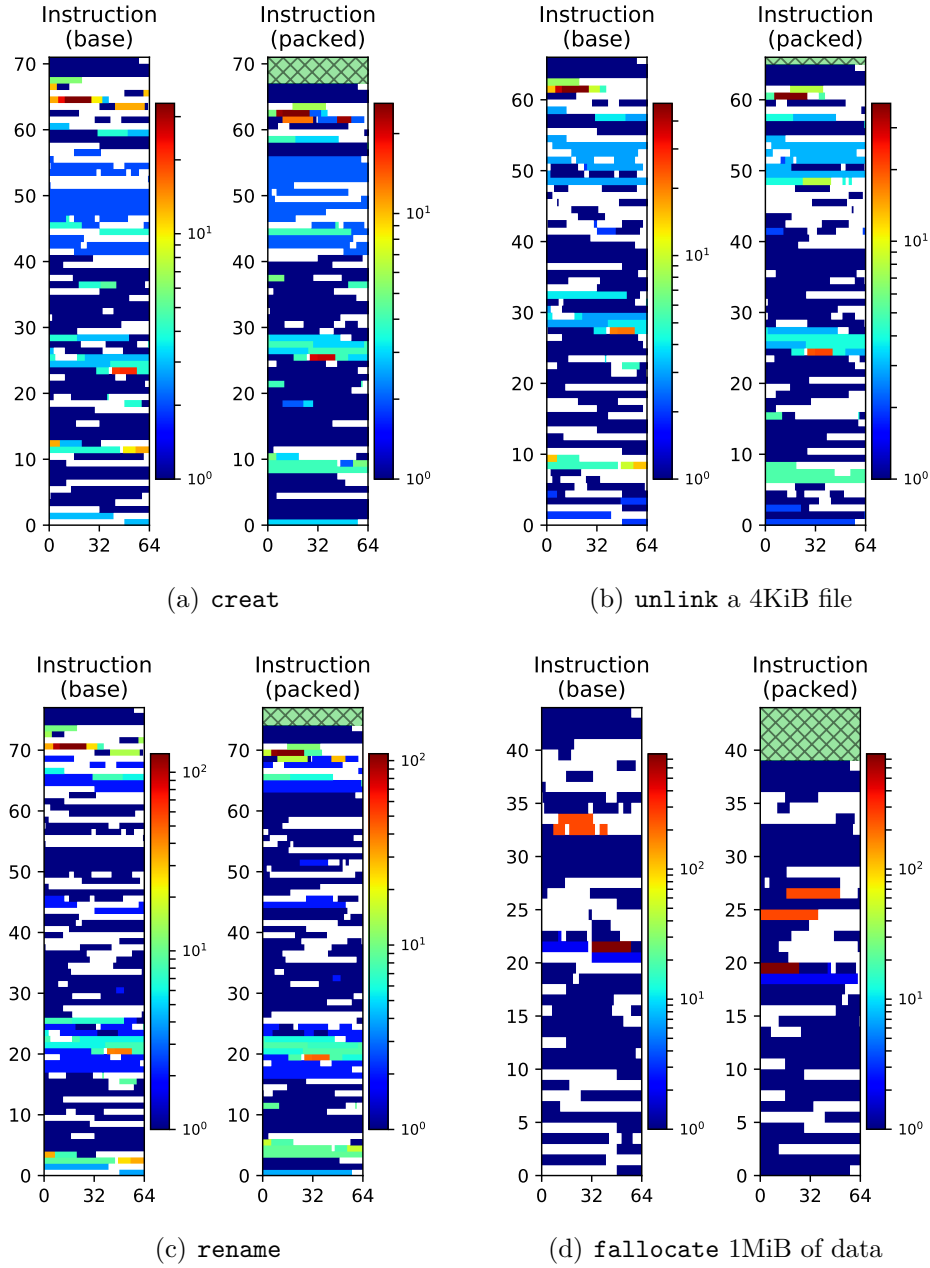
Figure 4.10: Instruction cachemaps of DenseFS, before and after cache-compaction optimizations. The hatched green regions near the tops of the packed cachemaps indicate cache footprint eliminated by the optimizations described in Section 4.3.
