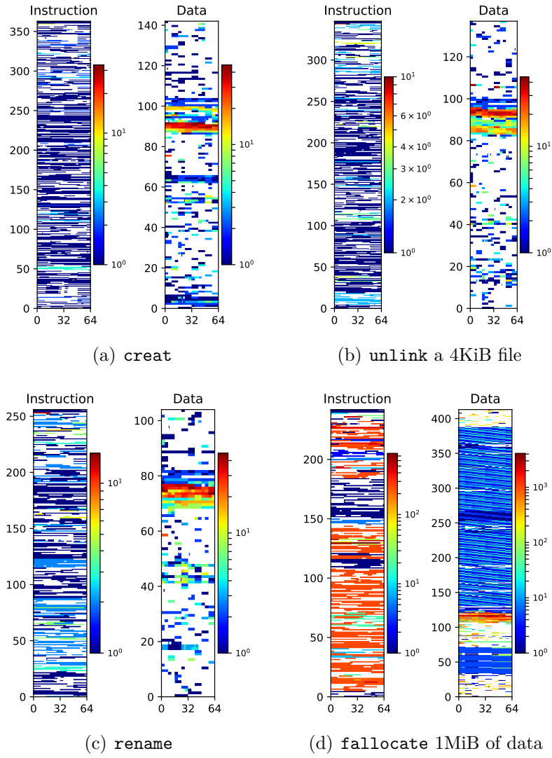
Figure 4.5: Cachemaps of metadata operations on tmpfs.
