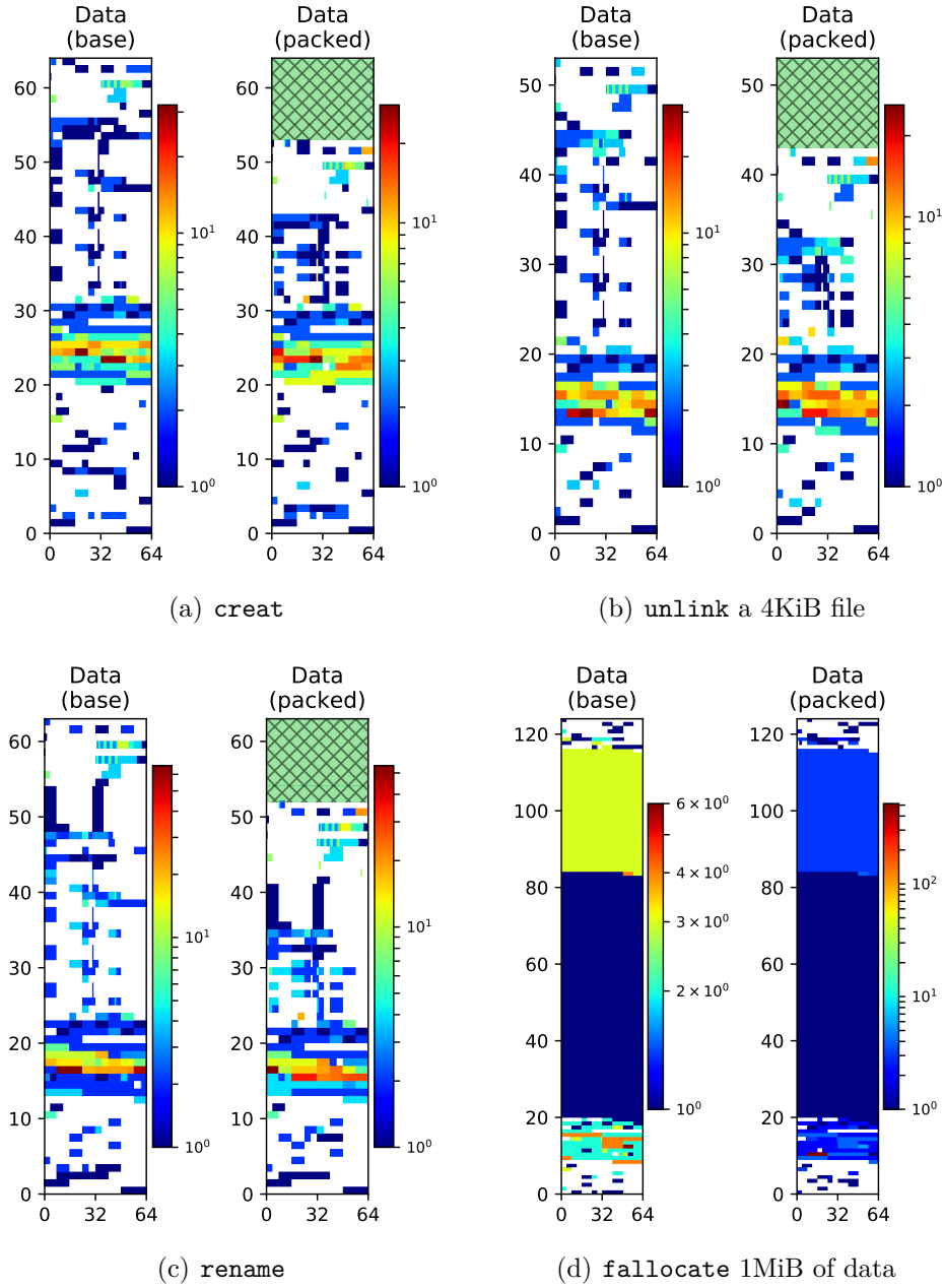
Figure 4.9: Data cachemaps of DenseFS, before and after cache-compaction optimizations. The hatched green regions near the tops of the packed cachemaps indicate cache footprint eliminated by the optimizations described in Section 4.3.
