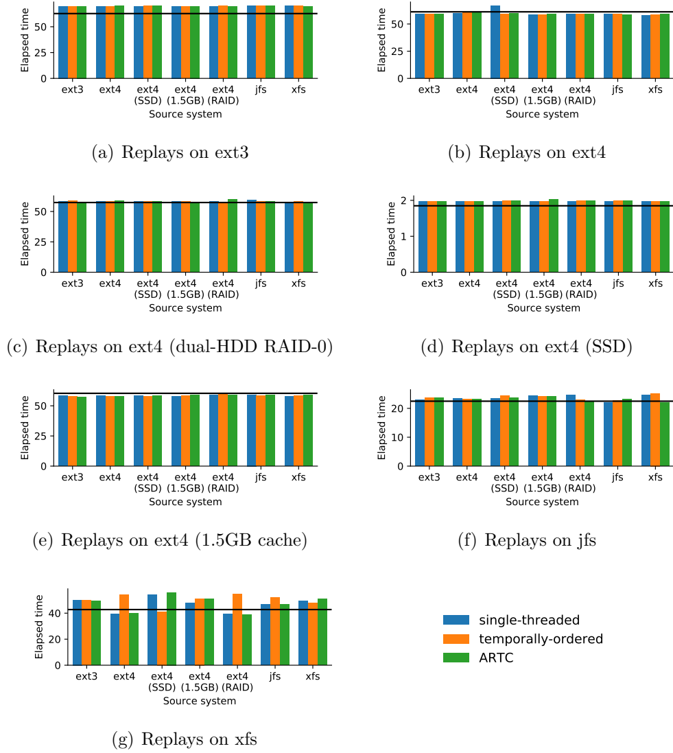
Figure 2.10: LevelDB fillsync replays. On each plot, a baseline shows how long the original program runs on the target platform. Bars near this line indicate an accurate replay.
