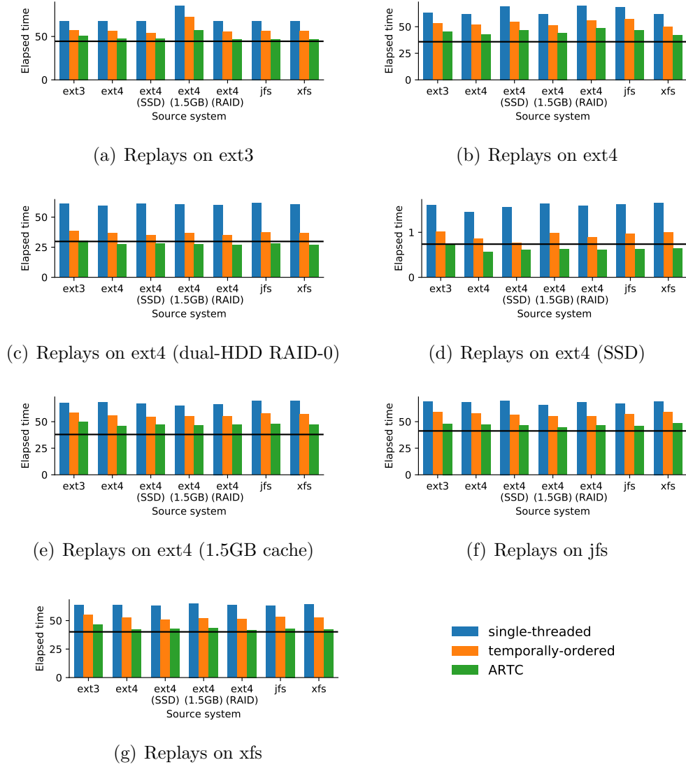
Figure 2.11: LevelDB readrandom replays. On each plot, a baseline shows how long the original program runs on the target platform. Bars near this line indicate an accurate replay.
