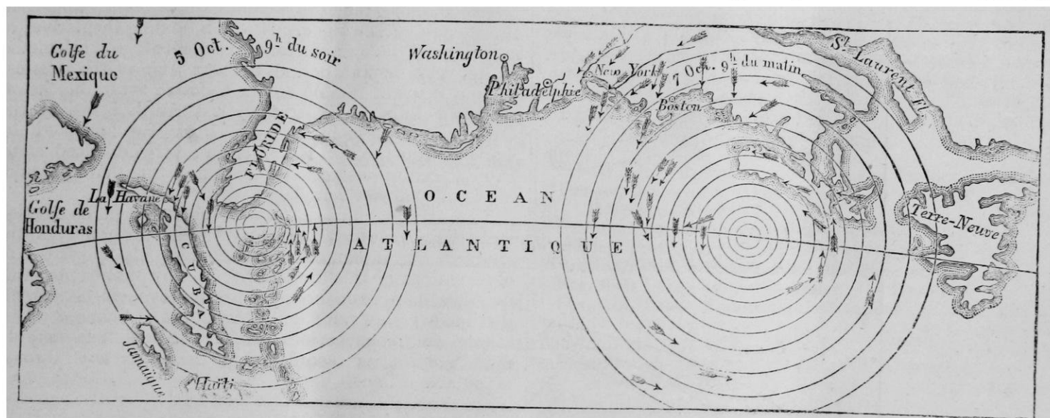
FIG. 1.—Hurricane at Cuba from Oct. 5 to 7, 1844.
