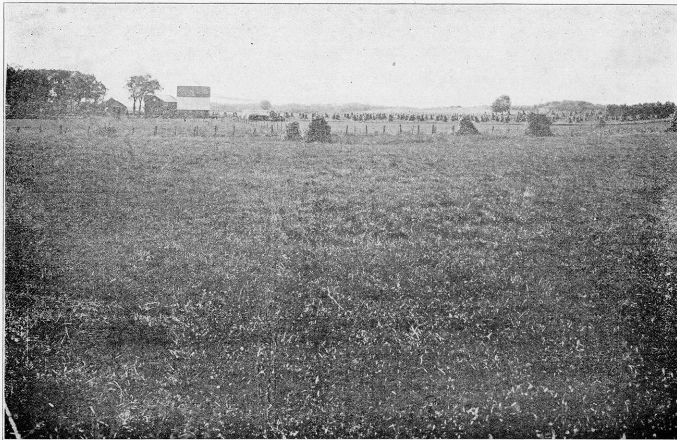
VIEW SHOWING LEVEL TO UNDULATING SURFACE OF WAUKESHA FINE SANDY LOAM AS IT OCCURS TO THE SOUTHEAST OF ONALASKA.
