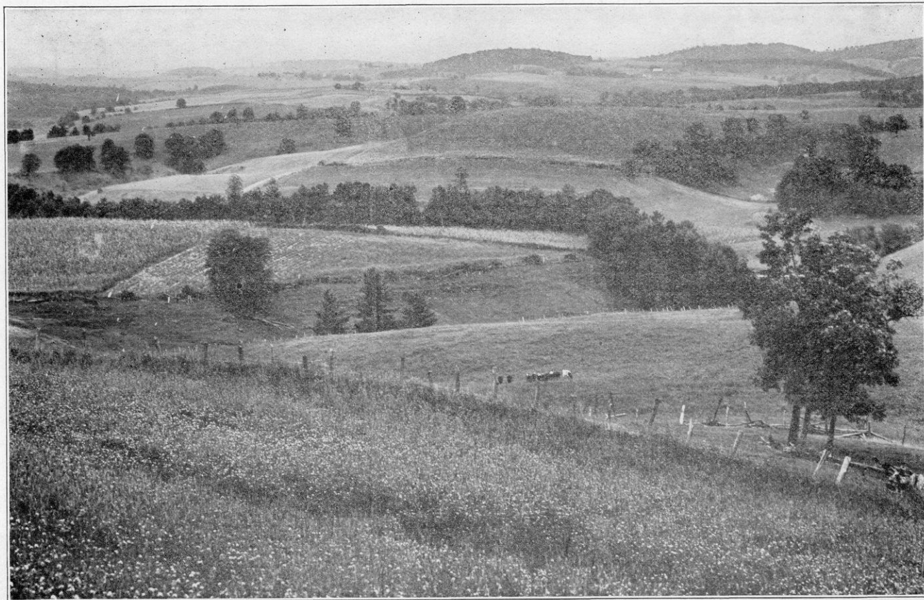
VIEW SHOWING CHARACTERISTIC TOPOGRAPHY OF KNOX SILT LOAM.
