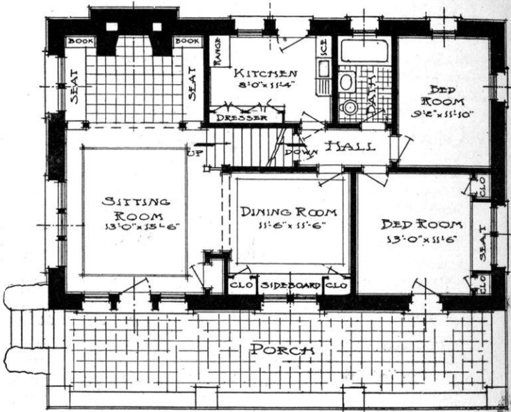
FLOOR PLAN OF STONE AND SHINGLE COTTAGE: NO. 93.
