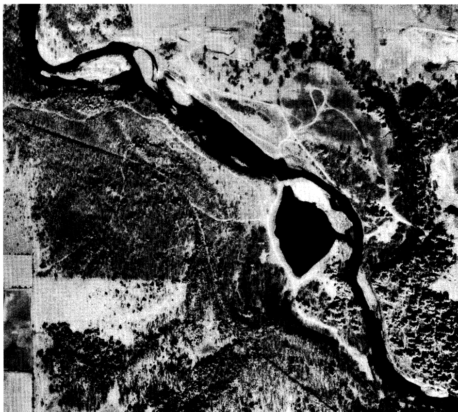
Figure 3. Aerial view of the dredged site (Station 4) and impacted site (Station 5) on the Big Rib River taken in 1987. Note the new channel formed upstream from the old dredged site, the formation of gravel bars and braided channel downstream from the new channel, the lack of flow over the old waterfall in the old channel, and the creation of a connected pond downstream from the old dredged site. The connected pond was formerly a flood-plain excavation site.
