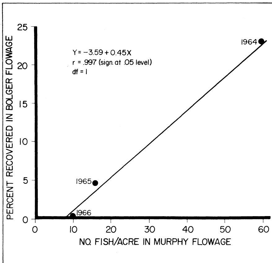
FIGURE 6. Relationship between population density and percent recoveries of stocked and native northern pike marked in Murphy Flowage in fall and recovered in Bolger Flowage the following spring, 1964-66.
