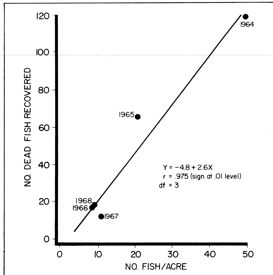
FIGURE 7. Relationship between standing crop and dead fish recovered during June 1964-68.
