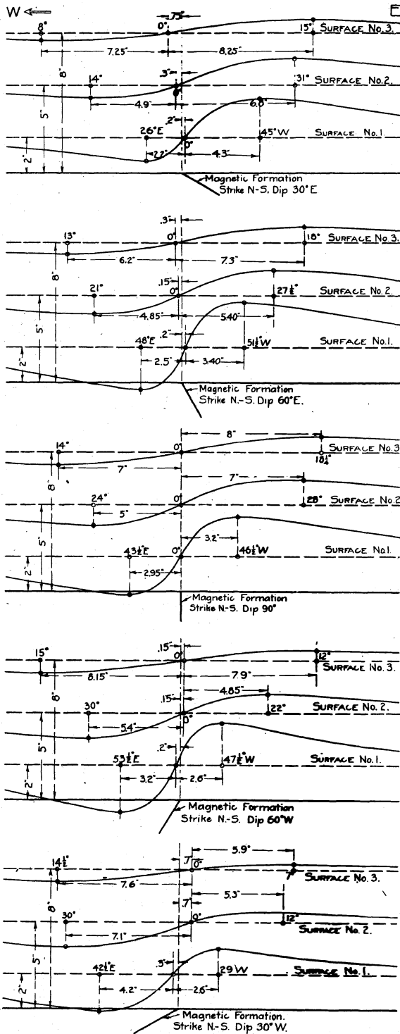
Fig. 24. Dial compass curves for N-S strike with various dips and depths of burial.
