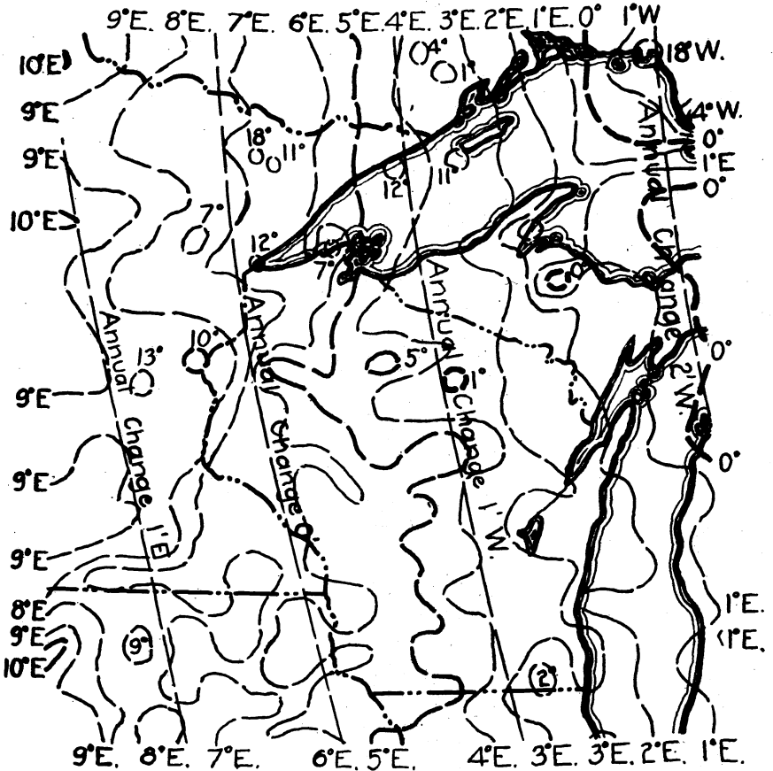
Fig. 4. Lines of equal declination and equal annual change. From U. S. Coast and Geodetic Survey chart.
