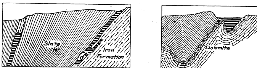
Fig. 36. Menominee Range. Cross sections showing occurrence of ore.
