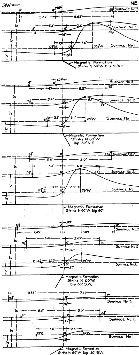
Fig. 26. Dial compass curves for strike N. 60° W. with various dips and depths of burial.
