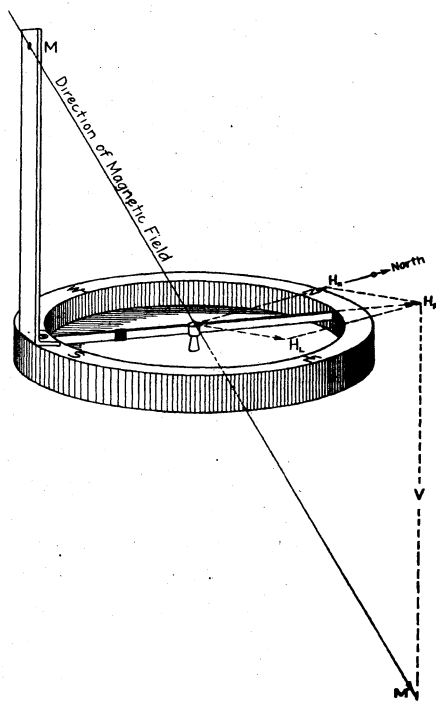
Fig. 20. The components of the earth's magnetic field usually considered are the vertical (V) and the horizontal (H R ). The horizontal component is often further divided into north (H N ) and local (H L ) components.
