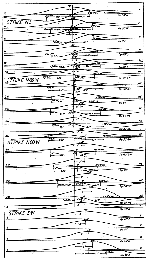
Fig. 27. Curves showing dial compass and dip needle readings for various positions of the iron sheet representing a magnetic formation.
