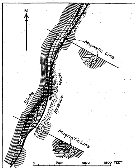
Fig. 38. Cuyuna Range. Plan showing relation of ore bodies and iron formation to the magnetic line.
