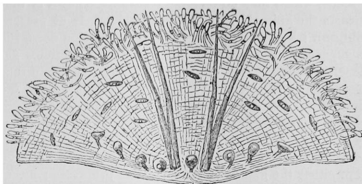
FIG. 8.— Utricularia neglecta . Valve of bladder; greatly enlarged.
