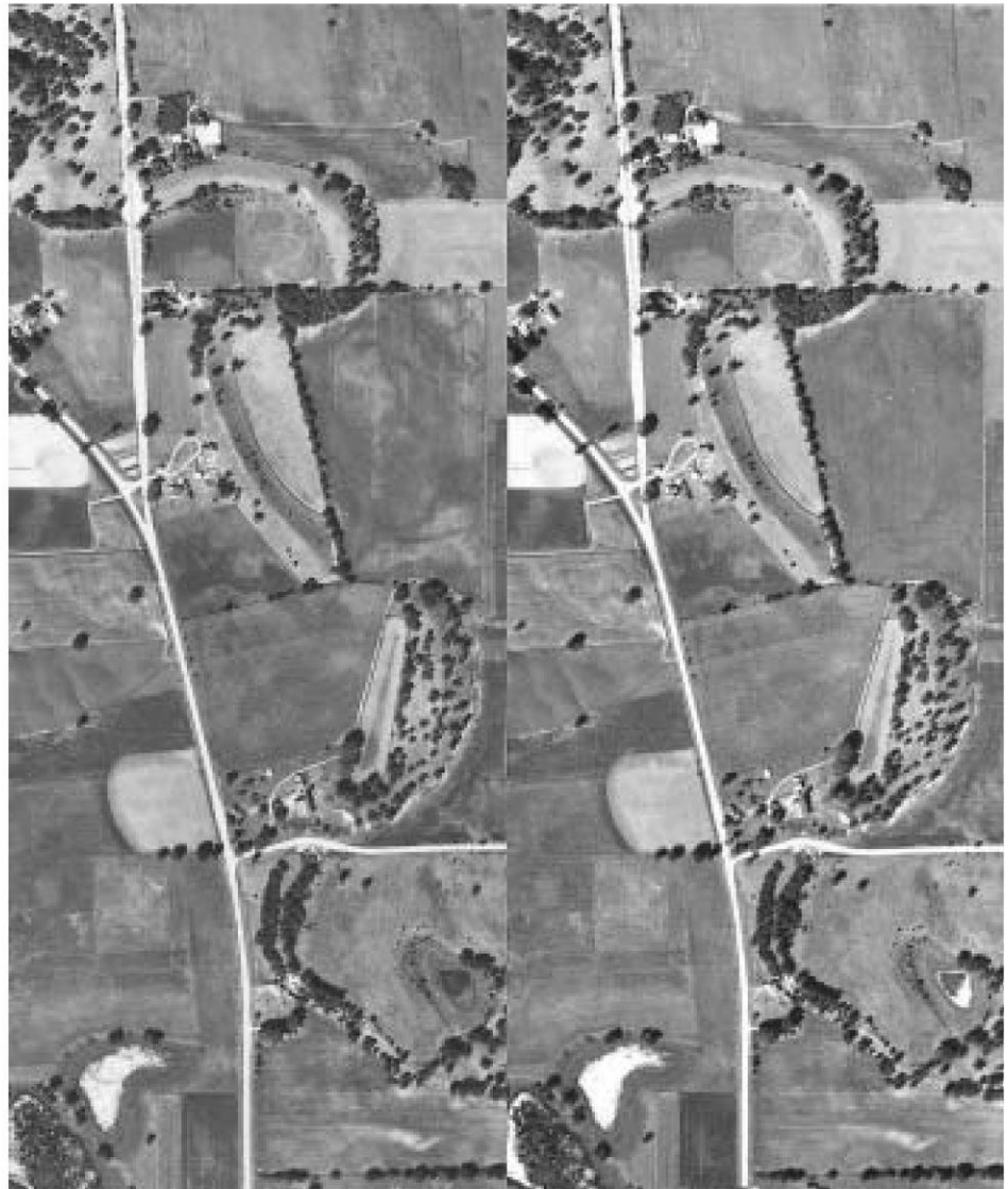
Figure 13. Stereographic pair of aerial photographs showing the esker-like ridge in the SE 1 / 4 sec. 29, T5N, R17E, southwest of Eagle. North is to the right. Area shown is 0.6 km from north to south. U.S. Department of Agriculture, Agricultural Stabilization and Conservation Service aerial photographs WW-2DD-31 and 32, August 20, 1963.
