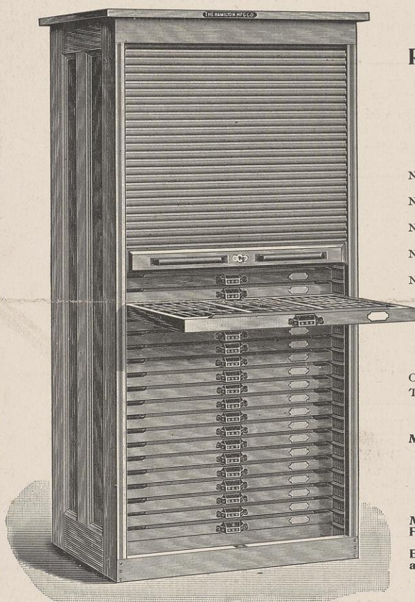
No. 5, ROLL FRONT CASE RACK. RACKS FOR 35 CASES. HEIGHT 83 INCHES.
